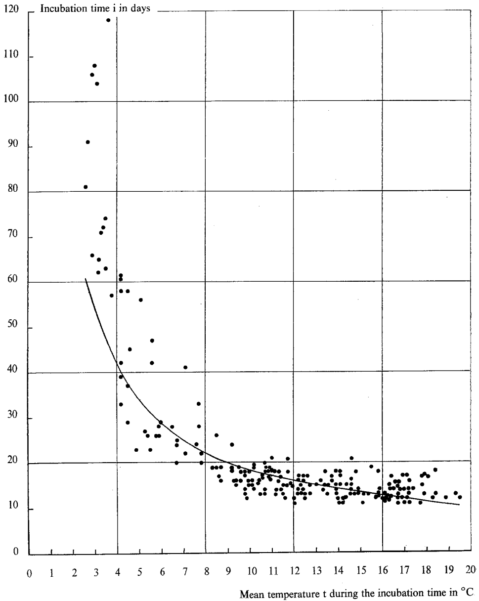
FIG. 32.2.a The relation between the incubation time i in days and the mean temperature t in ^{\circ}\text{C} . during the incubation time, over the years 1957–1960. The incubation time used is the “shortest observed incubation time”; dots represent individual observations at Wageningen. The mean temperature t is the mean temperature over the incubation time computed from hourly observations at the principle meteorological station in De Bilt. The regression line of fig. 32.2.b has been transformed into a reference curve.
