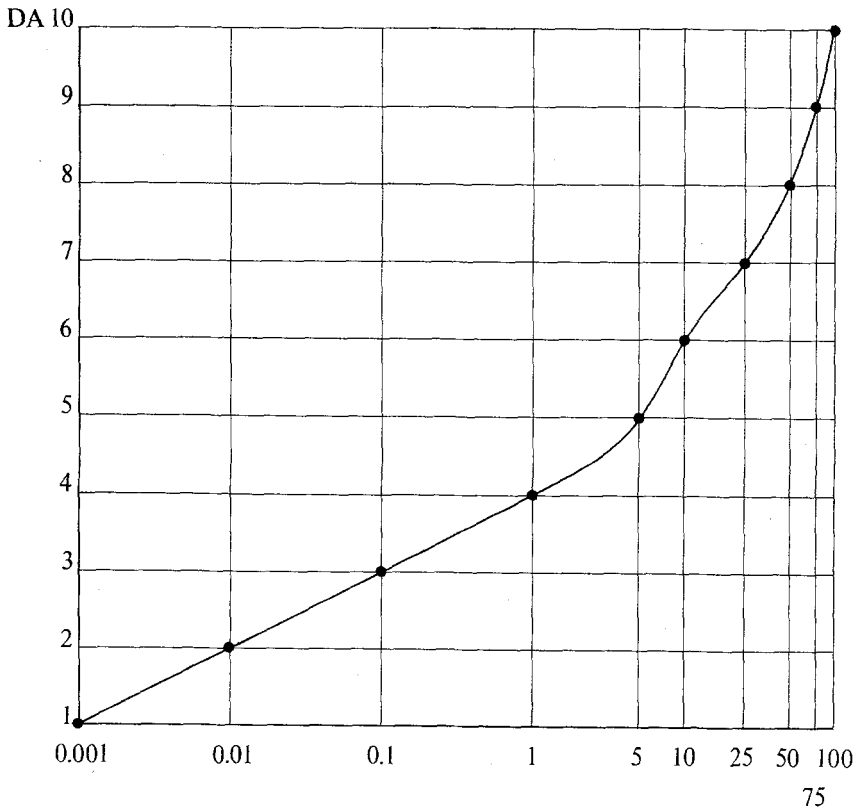
FIG. 24.24 The relation of the degree of attack DA to the percentage of attack PA. PA is plotted on a logarithmic scale, DA on a linear scale.
