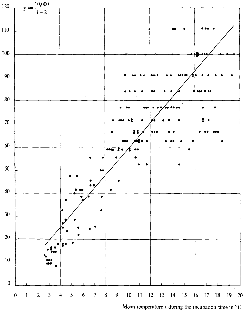
FIG. 32.2.b An empirical approximation of the relation between the incubation time i in days and the mean temperature t during the incubation time in °C., over the years 1957-1960. The regression line of y = \frac{10,000}{i-2} to t has been drawn; in fig. 32.2.a this regression line is transformed into a reference curve.
