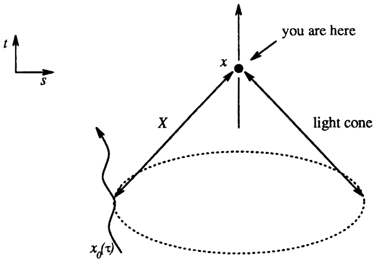
Fig. 2. A charge moving in the observer's past light-cone.
