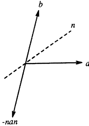
Fig. 1. A rotation composed of two reflections.
