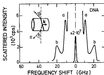
Fig. 1. Typical Brillouin spectrum of a dry semi-crystalline fibre of DNA recorded with a Fabry-Pérot interferometer using a free spectral range of 51 GHz in the scattering geometry ( \theta = 45^\circ ) as shown. The frequency shifts of the two doublets (a) and (b) were unambiguously determined by varying the free spectral range
