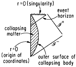
Fig. 2. A conformal diagram of a spacetime in which a body collapses and forms a black hole
