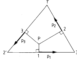
Fig. 1. Minimization of the potential energy in the case of a string interaction
