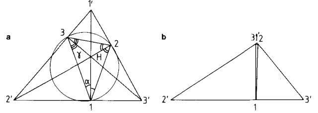
Fig. 2a, b. Minimization of the potential energy in the case of a sum of 2 body linear potentials. a The momenta form a triangle with all angles smaller than 90 degrees. b One of the angles is larger than 90 degrees.
