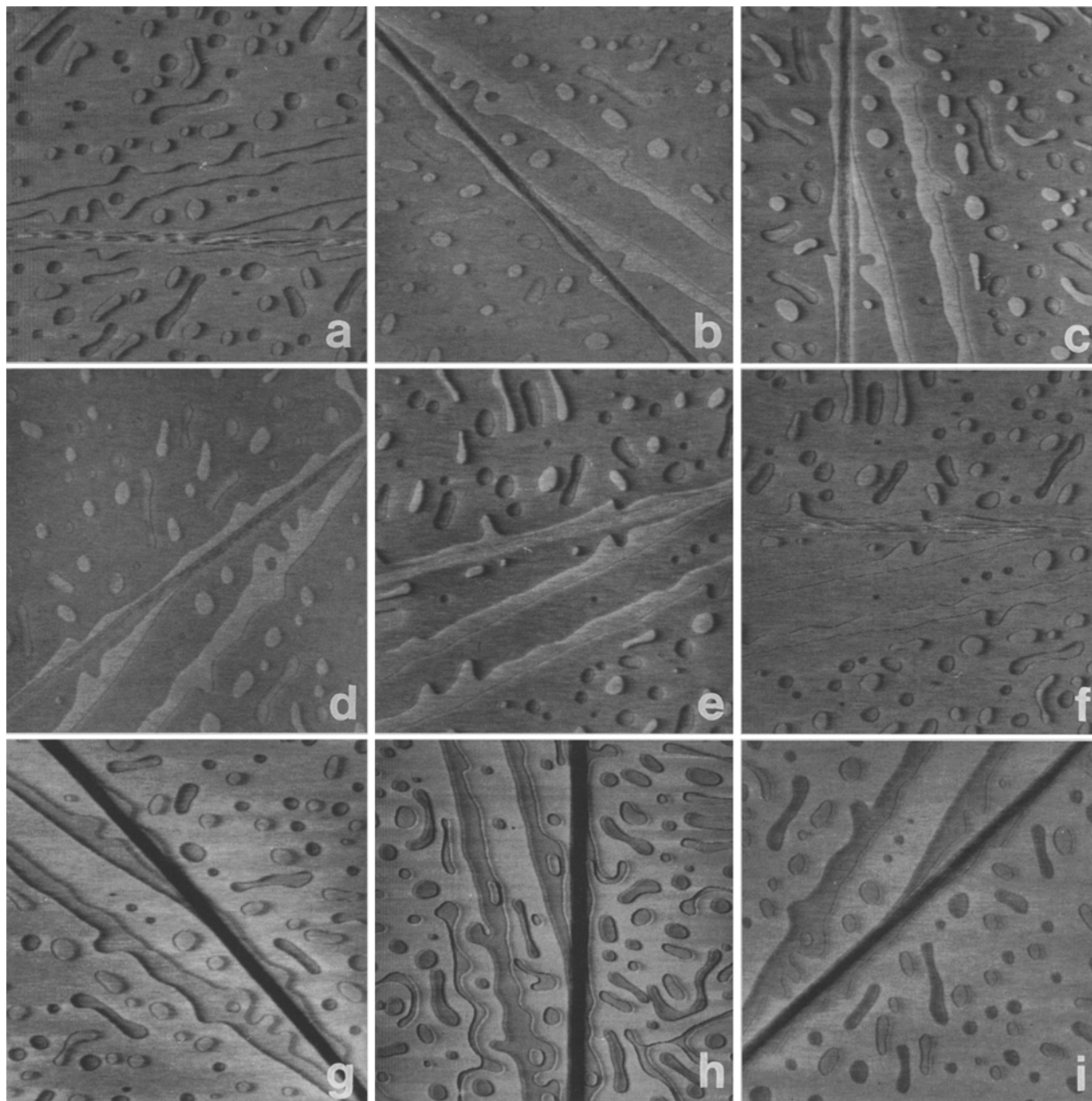
Fig. 7a-i. AFM images of a positive domain taken at the surface spot indicated in Fig. 2b. For the relative sample orientation and the cantilever scan direction see Fig. 8. The sample was successively
