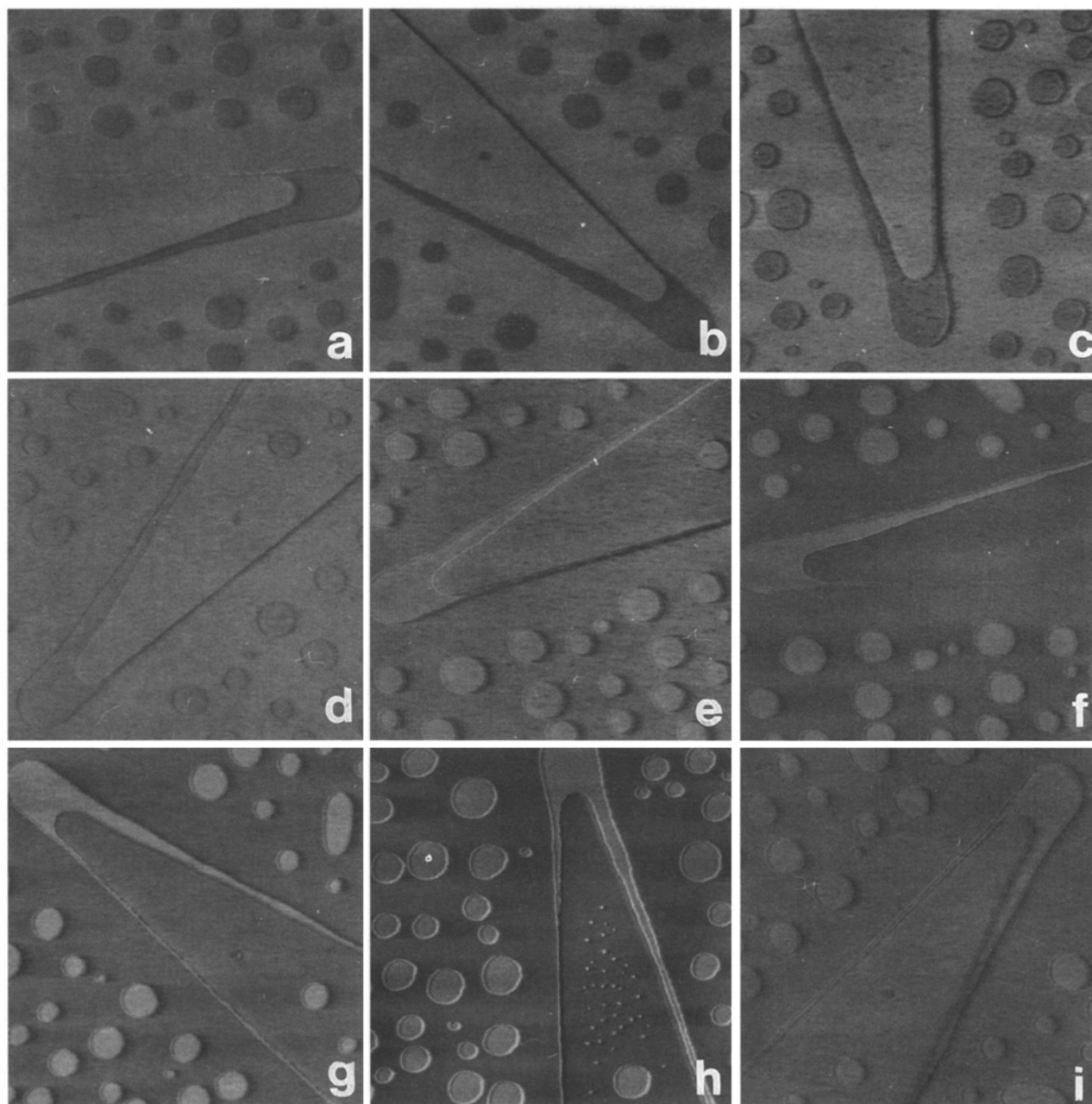
Fig. 6a–i. FFM images of a negative domain taken at the surface spot indicated in Fig. 2b. For the relative sample orientation and the cantilever scan direction see Fig. 8. The sample was successively
