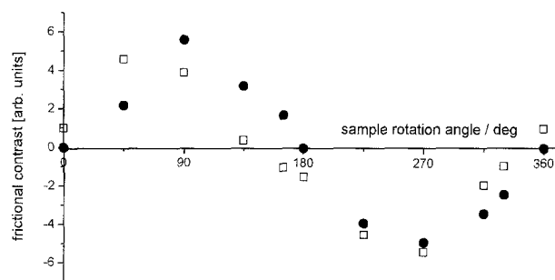
Fig. 9. Relative frictional contrast as a function of the sample rotation angle. A phase shift between the negative ( \square ) and positive ( \bullet ) domain by 15^\circ can be observed
