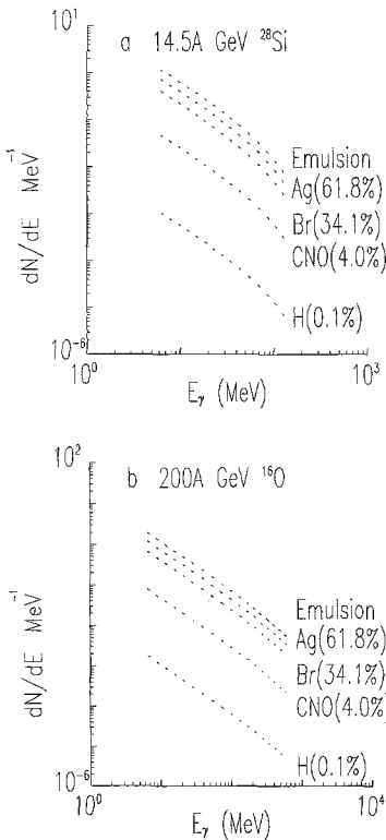
Fig. 1. The energy spectra of virtual photons for: a ^{28}\text{Si} beam at 14.5 A GeV and b ^{16}\text{O} beam at 200 A GeV in nuclear emulsion
