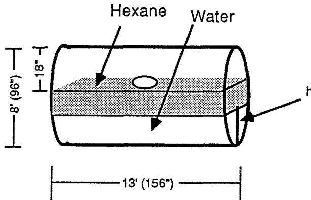
Fig. 8. A tank with water in the bottom and hexane sitting atop the water. The hexane always reaches the hole in the tank's side regardless of the height of the water.
