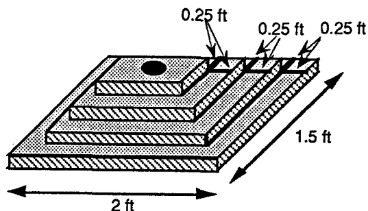
Fig. 3. A mold made of tiers with square bases. Each corner of a tier is offset 0.25 ft perpendicularly from the nearest edge of the tier below it.
