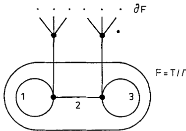
Fig. 9. The correspondence between rays in F = T/\Gamma and \mathbb{Q}_p -rational points of an algebraic curve ( g = 2, p = 3 ). The dots correspond to \mathbb{F}_p -rational points of the curve while the segments 1, 2, 3 correspond to double singular points (stable reduction)
