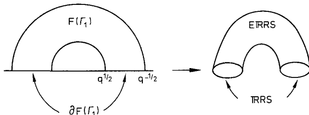
Fig. 1. Fundamental domains F(\Gamma_1) , \partial F(\Gamma_1) and the half-torus ( E\mathbb{R}RS ) in the archimedean case
