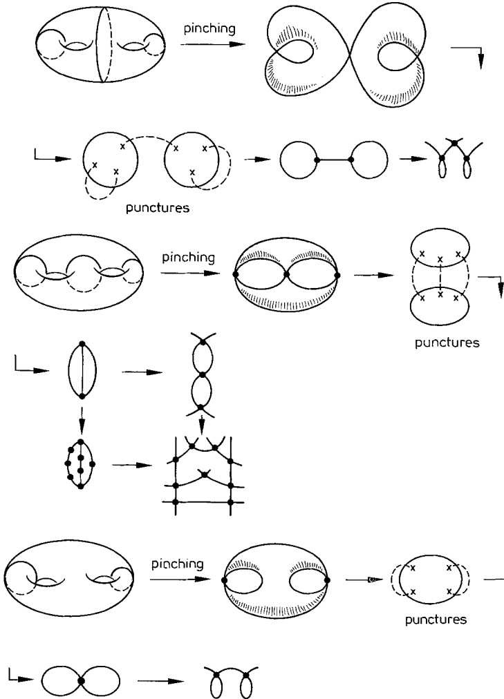
Fig. 10. Different types of degeneration for g=2 and corresponding reduced graphs. In b an example of semistable reduction is depicted. Dots in the reduced graph refer to the irreducible components P^1 which are depicted schematically as lines at the last picture of each sequence. Their intersections correspond to the edges in the reduced graph
