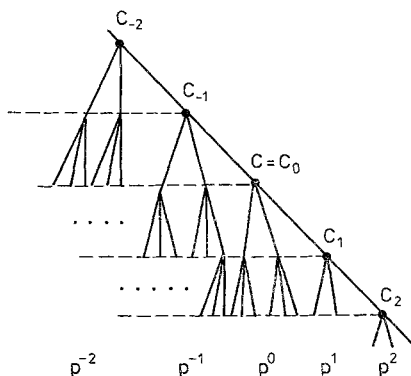
Fig. 12. The correspondence between rays and numbers
