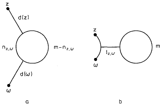
Fig. 5. The various mutual positions of the reduced graph F_1^R and the path z \rightarrow w
