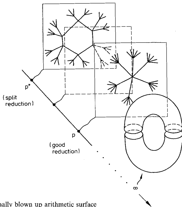
Fig. 11. Maximally blown up arithmetic surface
