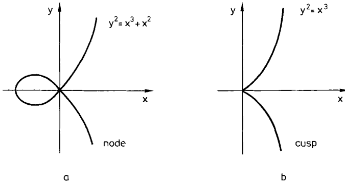
Fig. 8. Examples of singularities (elliptic curves over \mathbb{R} )
