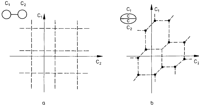
Fig. 13. The Voronoi decomposition in two dimensions
