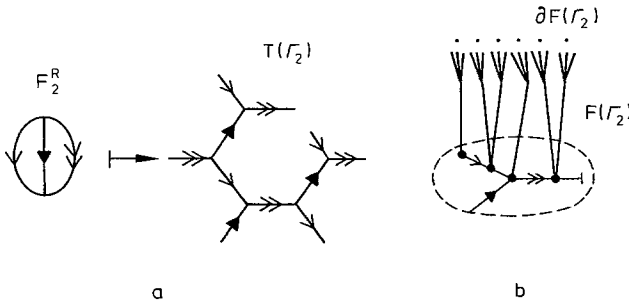
Fig. 14. An example of the Schottky tree T(\Gamma_2) . The choice of the connected fundamental domain F(\Gamma_2) leads to trivialization of the Prime form (B.5)
