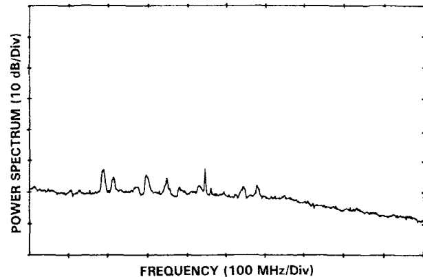
Fig. 4. Spectrum analyzer display of the beat note between the line-narrowed TDL and a CO laser, achieved with a MIM diode (single sweep, sweep time: 10 ms/div, resolution bandwidth: 1 MHz). The signal consists of many chaotic hopping lines; this points to uncontrolled optical feedback from the MIM diode to the TDL which de-stabilizes the diode laser
