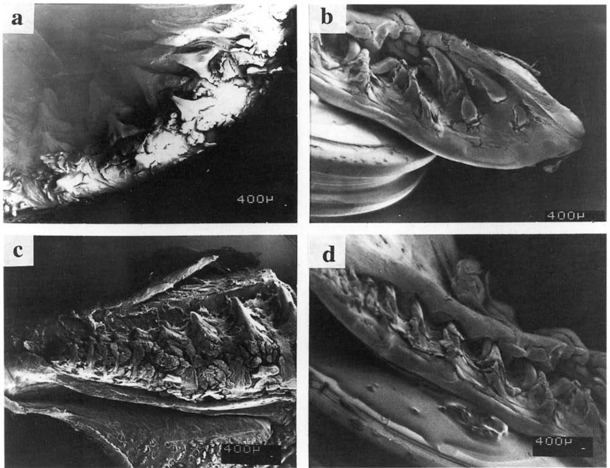
Fig. 8. a – SEM of dentition of 53.6cm TL embryo of C. taurus (HBOM 103:00264) revealing multiple tooth rows of anterior-most teeth (symphysis to upper right) and change in tooth morphology between rows. b – SEM of dentition of 48cm TL I. oxyrinchus embryo (HBOM 103:00250) showing multiple rows of anterior teeth (symphyseal teeth to right) and membranous sheath over teeth partially exposed by SEM preparation. c – SEM of (a) showing posterior lateral tooth rows. d – SEM of (b) showing posterior lateral tooth rows.
