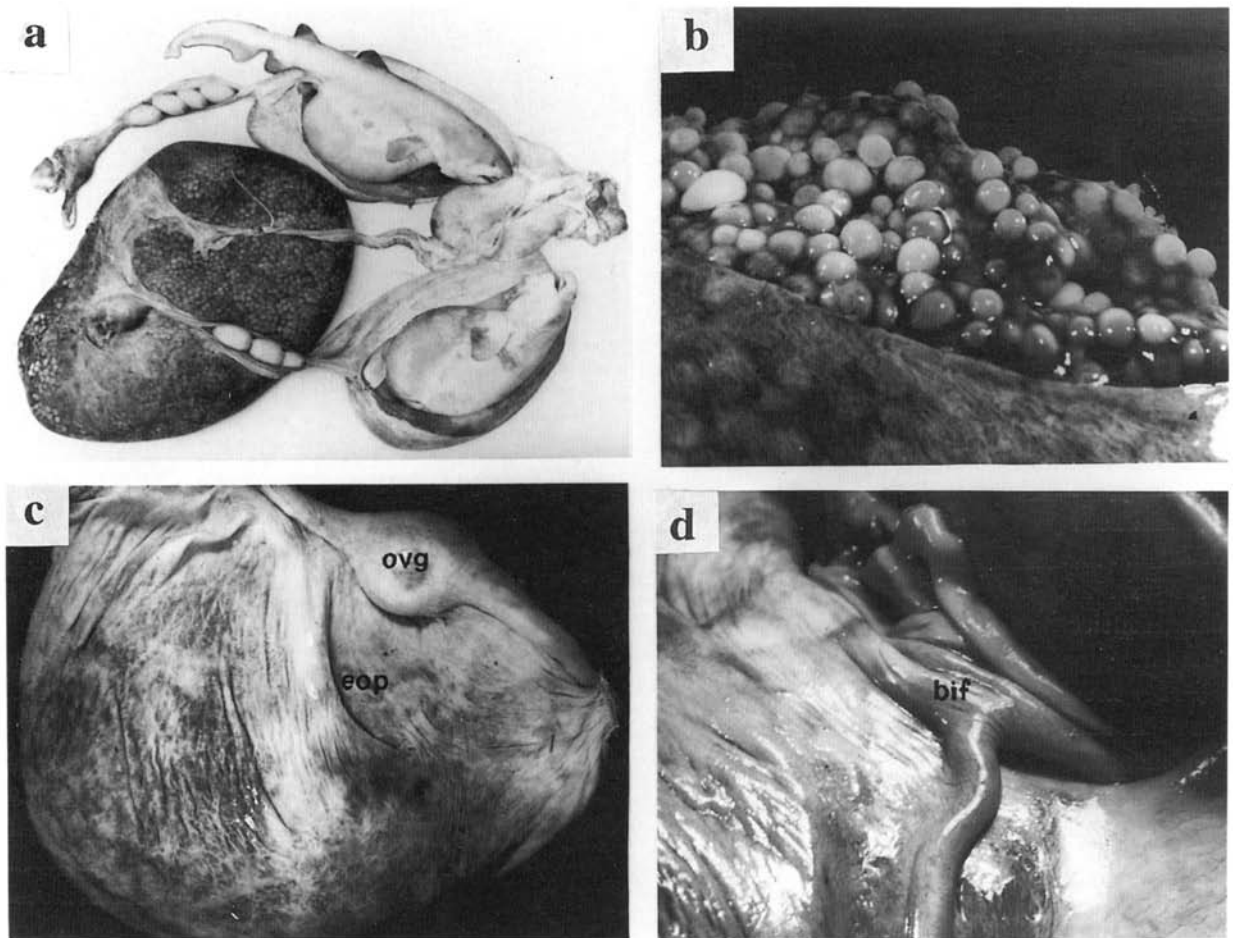
Fig. 4. a – Ovary, paired oviducts with egg capsules and oviphagous embryos of Carcharias taurus captured off Stuart, Florida, September 1989. Note nearly identical position and number of capsules in each oviduct. Photo courtesy of José Castro. b – Ova up to 10mm in diameter in ovary with membrane excized for exposure, C. taurus . c – Ovary of pregnant Isurus oxyrinchus (HBOM 103:00253) showing efferent ovarian pore (eop) and oviduct including the oviducal gland (ovg). d – Anterior oviduct of Carcharodon carcharias showing bifurcation (bif) of oviduct a few centimeters posterior to the ostium (to the right) at the liver.
