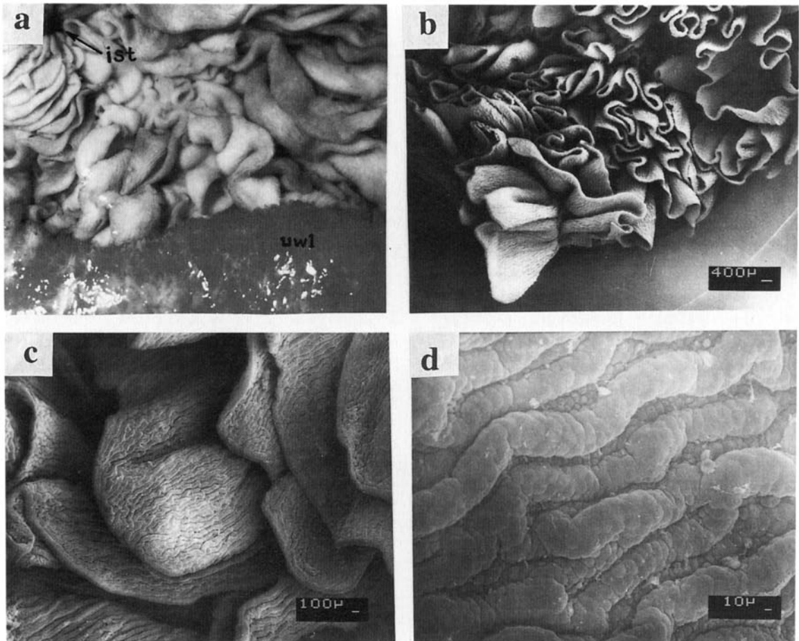
Fig. 5. a – Uterine membrane at isthmus (ist) with isthmian folds readily differentiated from remainder of uterine wall (uwl) with trophophemata in pregnant Isurus oxyrinchus (HBOM 103:00250). b – Scanning electron micrograph (SEM) enlargement of microfolds located on the isthmian folds photographed in (a). c – SEM enlargement of (b) showing ridges on microfolds. d – SEM enlargement of (c) showing detail of microfold ridges.
