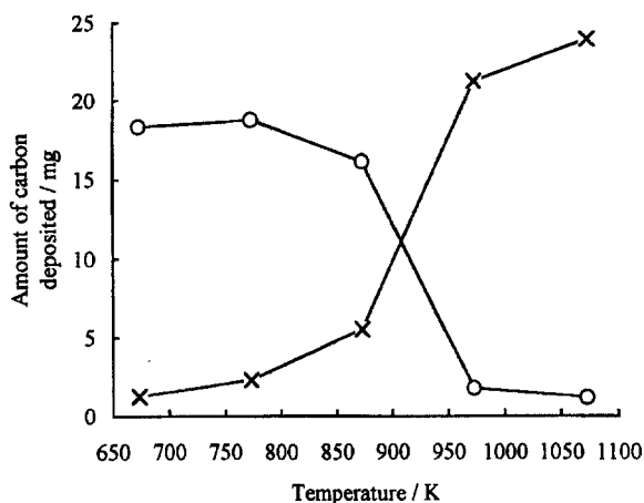
Fig. 3. The effect of temperature on the amount of carbon deposited from pure methane and pure carbon monoxide. Catalyst amount = 50 mg, flow rate = 8 ml min -1 , for 10 min. (×) CH 4 ; (○) CO.
