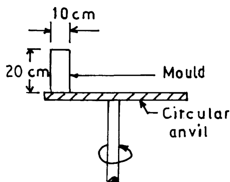
Figure 1 The mechanical rotating device.
