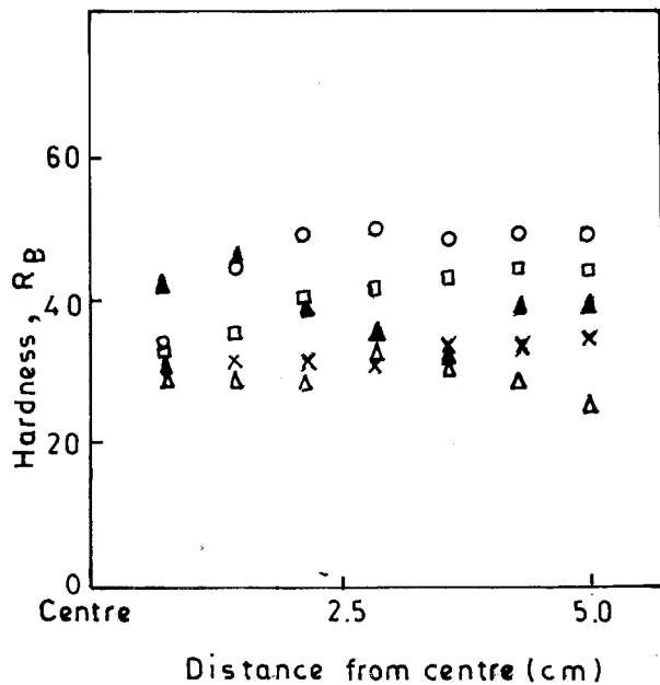
Figure 6 Variation of hardness with distance from the centre. Rotational speed: (○) 0, (□) 42, (×) 61, (△) 93 and (▲) 113 r.p.m.
