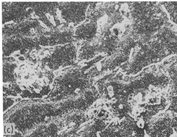
Figure 5 SEM micrographs of (a) edge at 93 r.p.m., (b) centre at 93 r.p.m., (c) edge at 113 r.p.m. and (d) centre at 113 r.p.m. ( \times 300 ).
