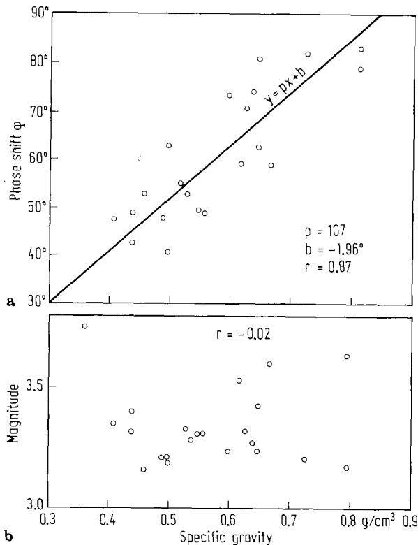
Fig. 2. Variation of a) the phase shift, b) the magnitude, with specific gravity
