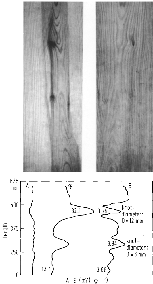
Fig. 5. Knot detection in pine ( Pinus pinaster )
