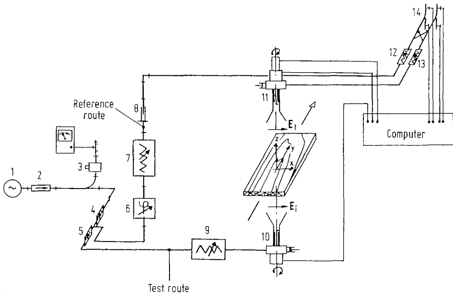
Fig. 1. Scheme of the set-up. 1 source (9,245 Mhz); 2 mono-directional line; 3 wavemeter; 4; 5; 7; 12; 13 attenuator; 6 calibrated static phase shifter; 8 sliding linkage; 9 calibrated attenuator; 10; 11 antenna; 14 measuring head
