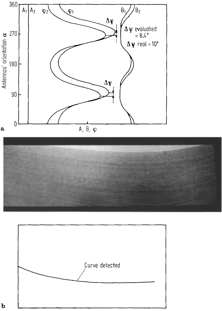
Fig.4. a Slope of the grain evaluation between two points; b Oak; mean slope of grain evaluation
