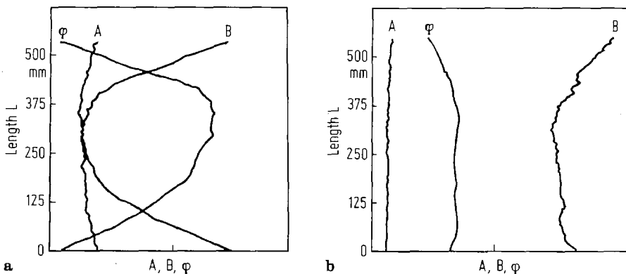
Fig. 3. Variation of B (mV) and phase shift \varphi (°) along the board length L . Analysis at different times a) 26. 8. 83 and b) 22. 9. 83
