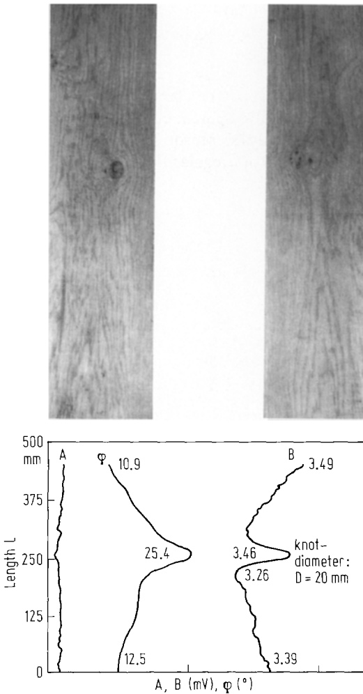
Fig. 6. Knot detection in oak
