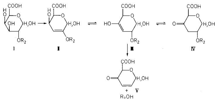
Fig. 3. Proposed route for the alkaline degradation of 2-O-( \alpha -L-rhamnopyranosyl)-D-galacturonic acid. R 2 represents the rhamnose group in the xylan chain. For simplicity only one isomer has been included
