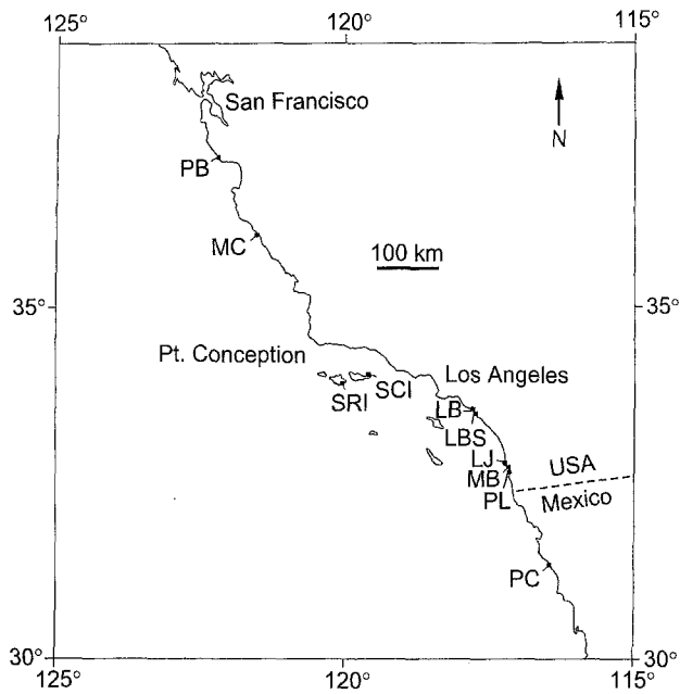
Fig. 1 Location of collection sites in California, USA, and Baja California, Mexico (PB Panther Beach, May 1995; MC Mill Creek, May 1995; SCI Scorpion Anchorage, Santa Cruz Island, July 1994; SRI Ford Point, Santa Rosa Island, November 1994; LB Laguna Beach, January 1995; LBS Laguna Beach South, March 1995; LJ La Jolla, September 1994; MB Mission Bay, March 1994; PL Point Loma, October 1994; PC Punta Cabras, October 1994)
