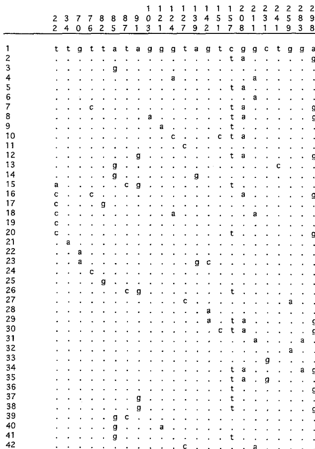
Fig. 2 Strongylocentrotus purpuratus . Nucleotide variation in 42 mitochondrial DNA haplotypes (Numbers on top abscissa nucleotide positions; dots positions identical to Haplotype 1) Position 1 corresponds to Position 6390 in sequence published by Jacobs et al. (1988)
