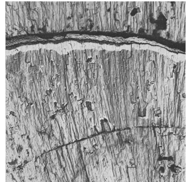
Fig. 8. Electronmicrograph of otolith of Aplodinotus grunniens (platinum-carbon replica)
