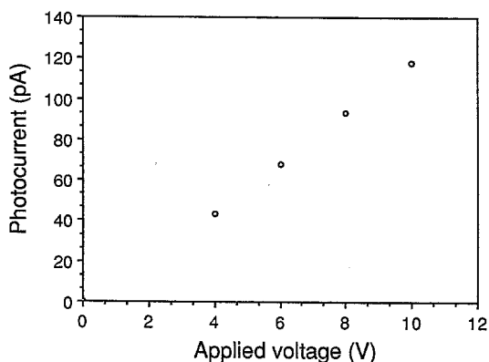
Fig. 4. Photocurrent measured as a function of bias voltage at 514 nm with laser intensity of 0.3 W/cm 2
