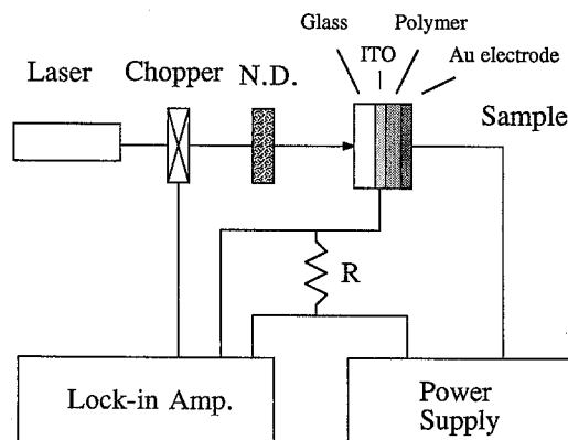
Fig. 2. Experimental set-up for photoconductivity measurement
