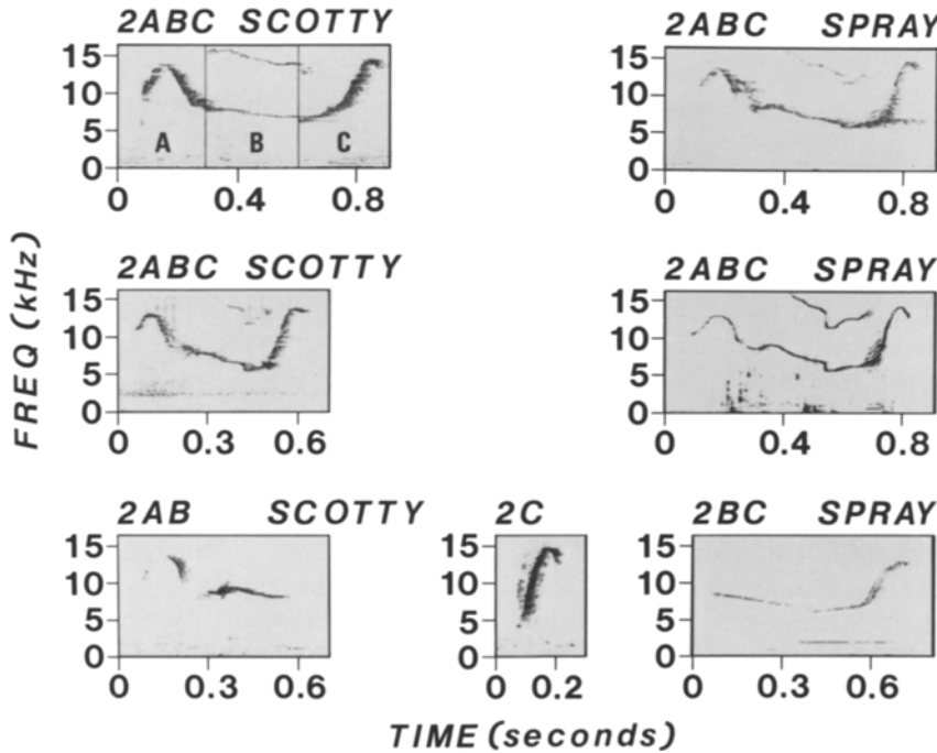
Fig. 2. Spectrograms of Type 2 whistles. The whistles on the left were all produced by Scotty; those on the right were produced by Spray. Type 2 whistles were formed of three segments, 2A, 2B and 2C. These are separated by vertical lines in the spectrogram on the upper left of the figure. The top two rows show complete type 2 whistles, while the bottom row shows whistles that included only one or two of these segments
