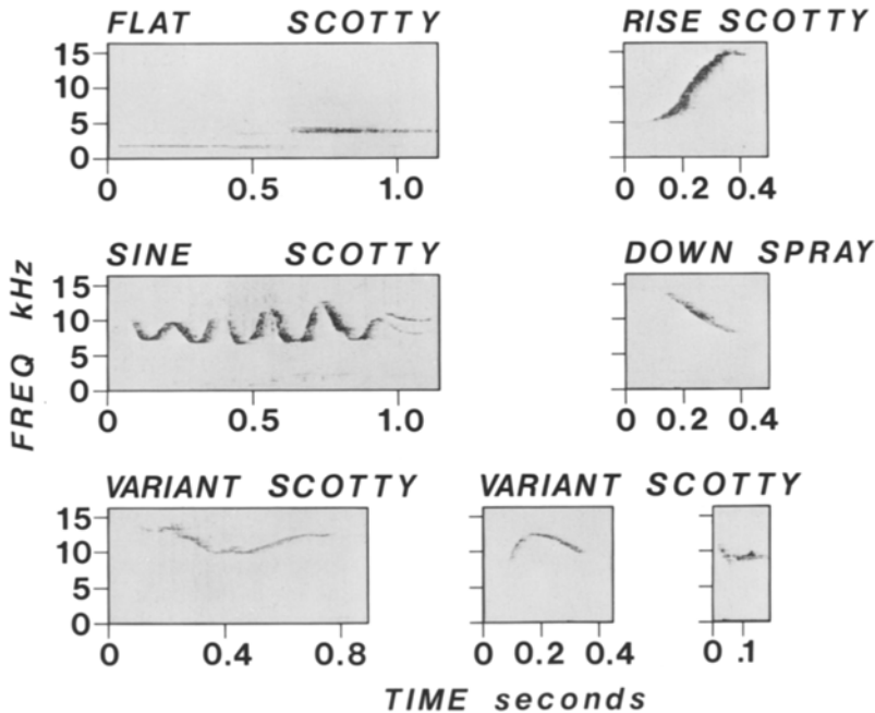
Fig. 3. Spectrograms of secondary whistle contours. The first half of the spectrogram on the upper left shows a 1.5 kHz signal from the trainer's whistle, while the second half shows a FLAT whistle of approximately 3 kHz produced by Scotty. The rest of the spectrograms all show examples of secondary whistles produced by Scotty, except for the DOWN whistle on the middle right, which was produced by Spray
