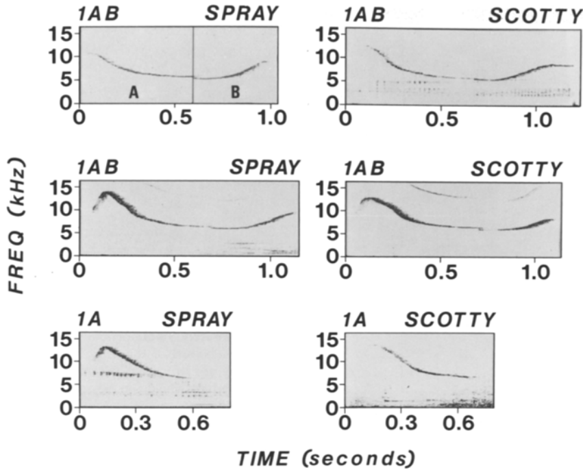
Fig. 1. Spectrograms of Type 1 whistles. The whistles on the left were all produced by Spray; those on the right were produced by Scotty. Type 1 whistles were formed of two segments, 1A and 1B. These are separated by a vertical line in the spectrogram on the upper left of the figure. The top two rows show complete type 1 whistles, while the bottom row shows whistles that included only the 1A segment
