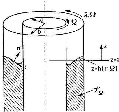
Fig. 1. The free surface between rotating cylinders
