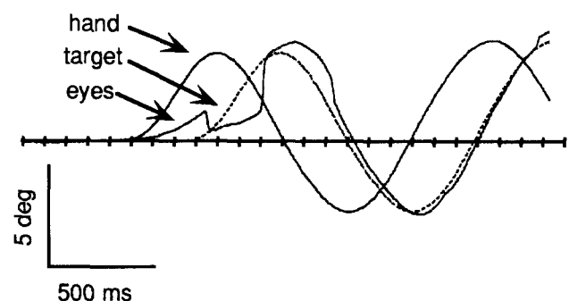
Fig. 8. Beginning of eye tracking of a target moved by the hand, with a 300 ms delay introduced in the visual feedback. Condition and conventions are the same as in Figure 7. Even when a large artificial delay is used (here 300 ms), the eyes always start to move with smooth pursuit in synchrony with the arm. The gain of this non-visual smooth pursuit is low (0.4), and a saccade is always triggered in the direction opposite to the arm motion
