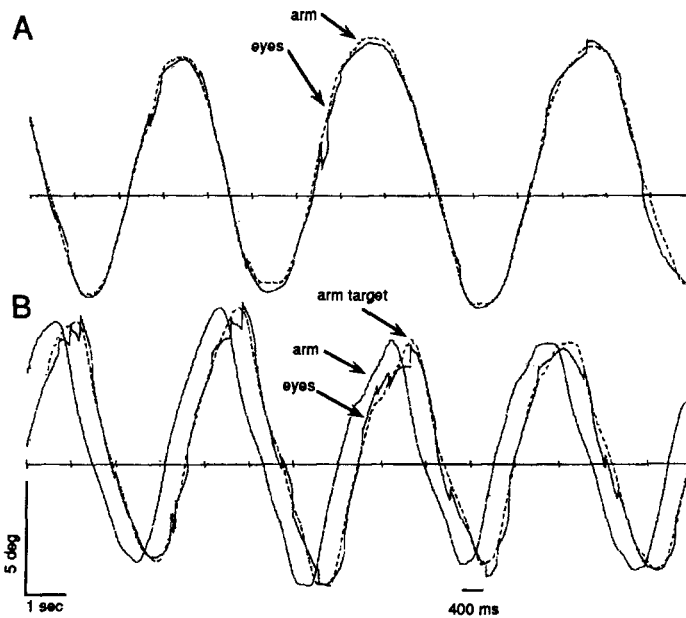
Fig. 4A, B. Typical ocular tracking of the arm-moved target without artificial delay (A) and with a 400 ms delay (B). The S is instructed to move his arm sinusoidally at a frequency of 0.2 or 0.5 Hz, over a \pm 5^\circ range. Traces representing arm and eye motions are essentially superimposed, showing good tracking performance in this condition. In B, the dashed line represents the arm-moved target motion, that is the arm motion shifted by 400 ms, while in A the dashed line represents the actual arm and target (delay = 0) motions. An enlarged view of traces shown in B is provided in Figure 6 to emphasize tracking characteristics when large artificial delays are used
