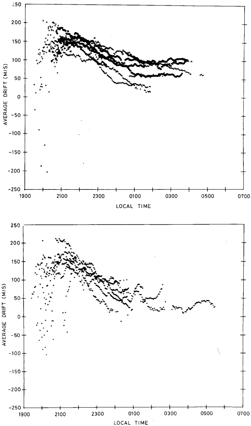
Fig. 12. (a) Local time variation of the average drift of equatorial F -region irregularities obtained from spaced receiver measurements of scintillations at Guam (magnetic dip 4.8^\circ N) for some magnetically quiet periods during summer solstice (crosses) and equinox (circles). (b) Same as (a) for seven magnetically disturbed days with \Sigma K_p \geq 30 (Bhattacharyya et al. , 1989).
