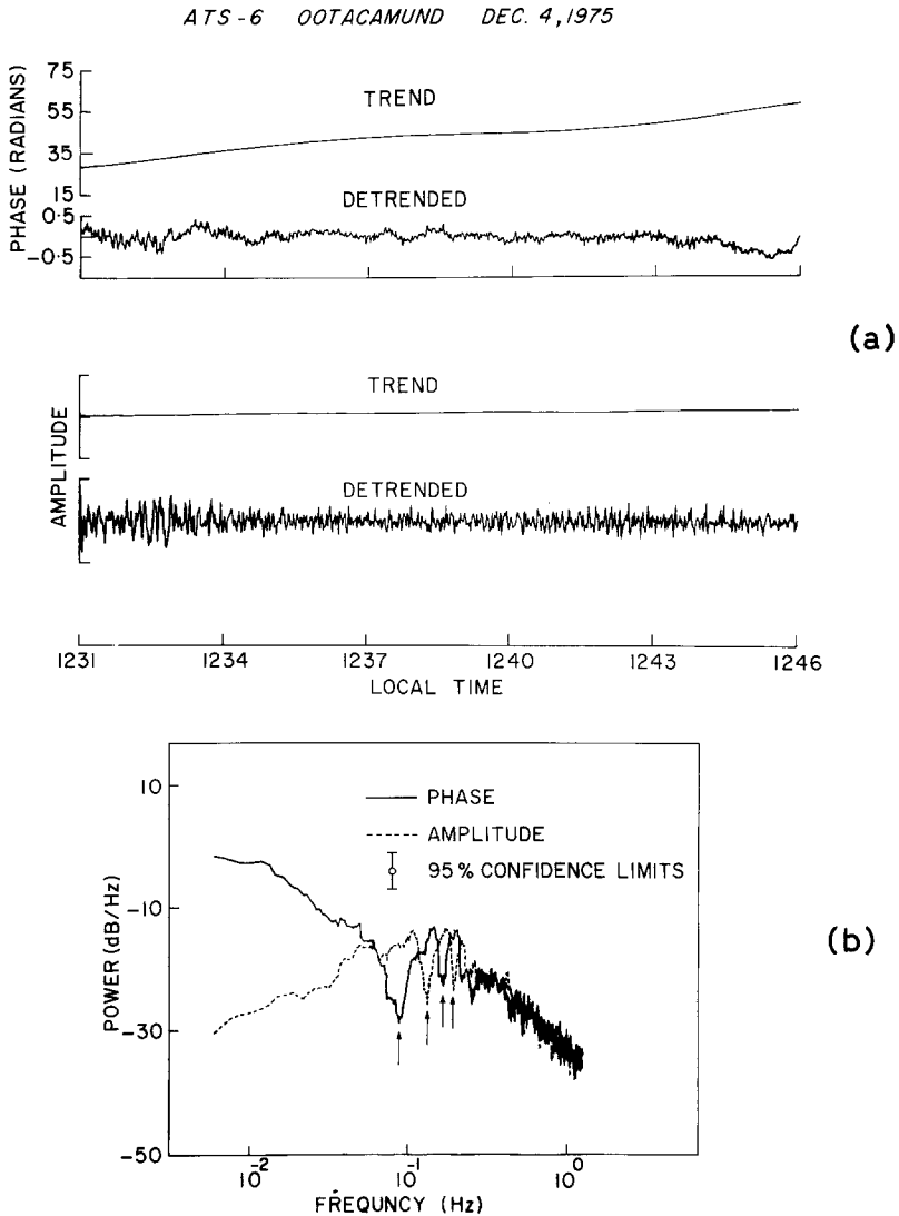
Fig. 3. (a) Detrended phase and amplitude scintillation data recorded at an equatorial station, Ootacamund (subionospheric dip 4.4^\circ N). (b) Smoothed power spectra of the detrended scintillation data. First few Fresnel minima are indicated by arrows (Bhattacharyya, 1991).
