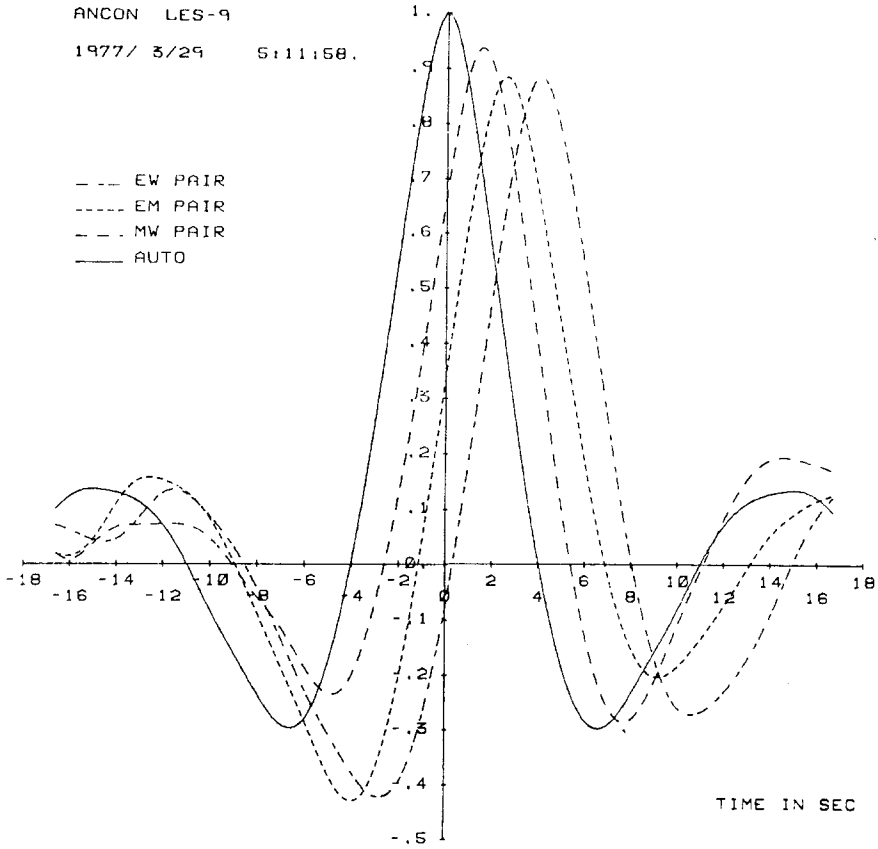
Fig. 10. Auto- and cross-correlation functions computed from amplitude scintillations on a 249 MHz signal, transmitted from LES 9 satellite and recorded at Ancon (11.71° S, 77.15° W) by three receivers aligned in the east-west direction (Wernik et al. , 1983).
