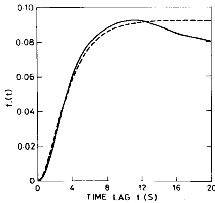
Fig. 15. (a) Phase trend, filtered phase, amplitude trend and filtered amplitude for a 140-MHz signal from the geostationary satellite ATS 6 received at the equatorial station Ootacamund during a period of weak to moderate scintillations ( S_4 = 0.48 ). (b) f(t) , which is related to the MCF through Equation (4.11), computed from data (solid line) and from theory (dashed line) (Bhattacharyya and Rastogi, 1991).
