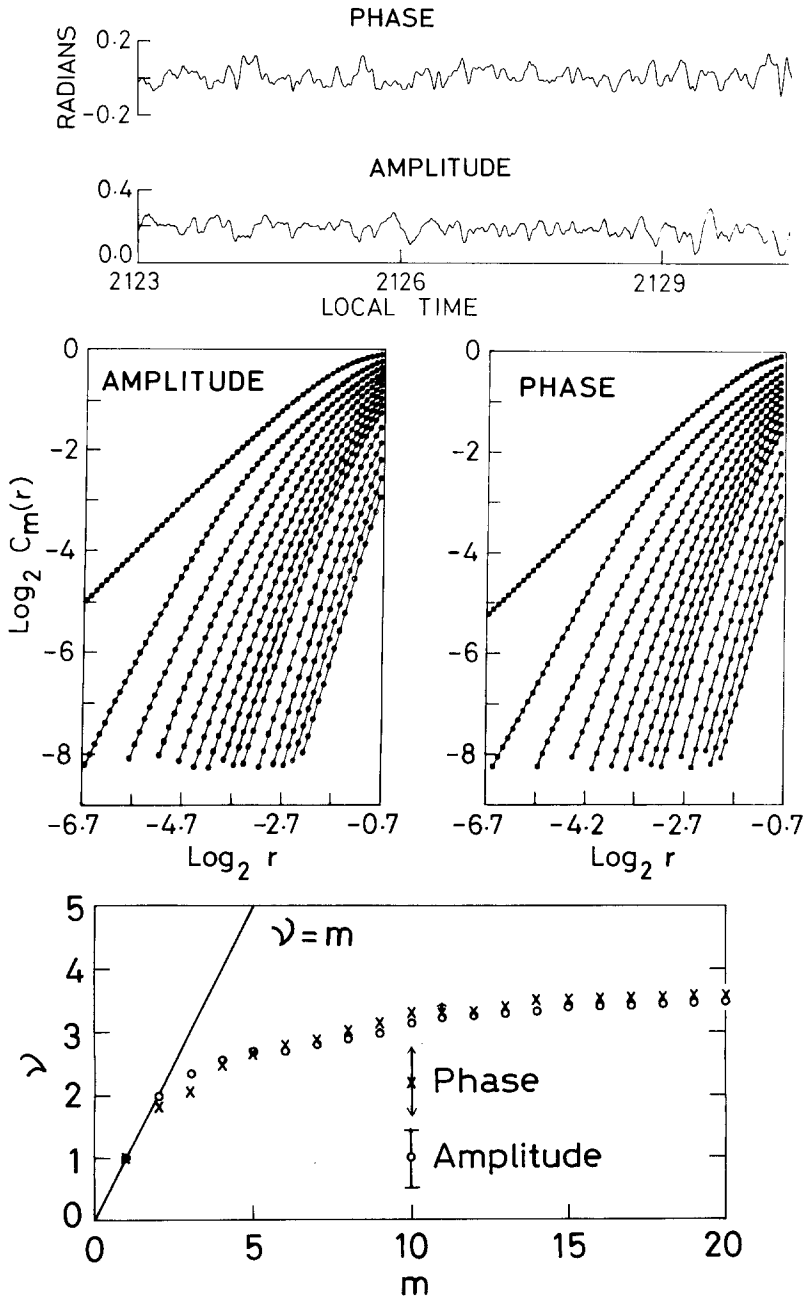
Fig. 18. (a) Filtered amplitude and phase scintillation data with S_4 = 0.36 and \sigma_\phi = 0.21 radians. (b) Plots of correlation integral C_m(r) computed from the data for embedding dimension m = 1 to 10, 12, 14, 16, 18, and 20 , starting from the left. (c) Slope \nu in the linear range of plots in (b) as a function of m . Purely stochastic behavior would yield the straight line \nu = m . Here \nu is seen to approach a constant value D_2 \approx 3.4 for sufficiently high values of m for both amplitude and phase data, indicating low dimensionality for the ionospheric density fluctuations (Bhattacharyya, 1990).
