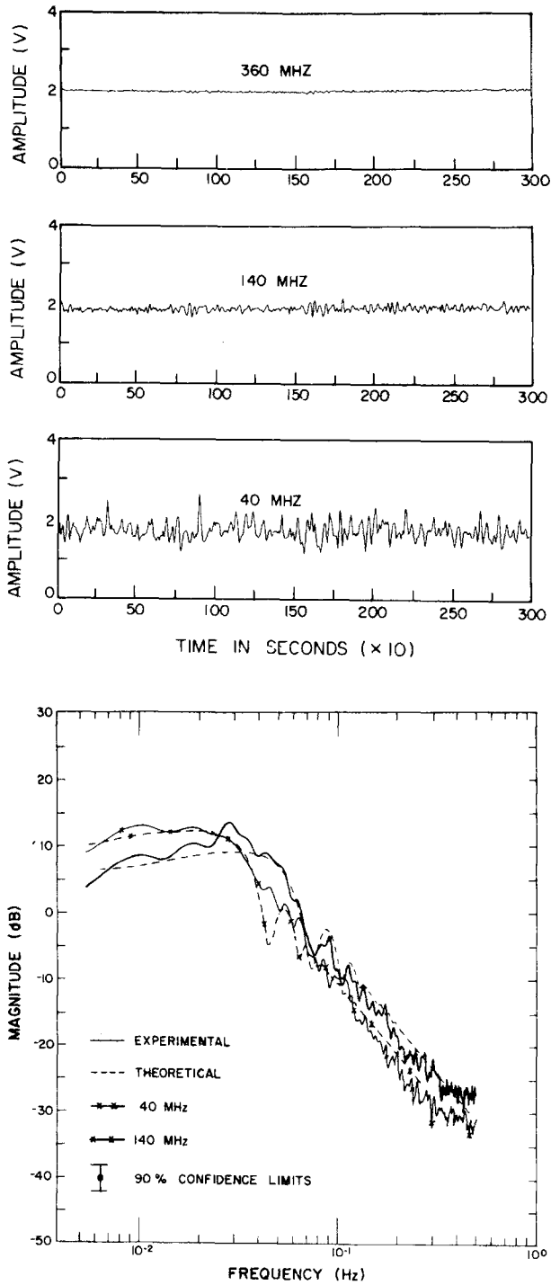
Fig. 2. (a) Amplitude scintillations on 40-, 140-, and 360-MHz signals from the ATS-6 satellite ( 94^\circ W) recorded at Boulder ( 40.13^\circ N, 105.24^\circ W).
