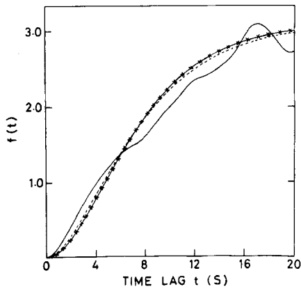
Fig. 16. (a) Same as Figure 15(a) during a later period when scintillations are strong ( S_4 = 0.90 ). (b) Same as Figure 15(b) for the data shown in Figure 16(a). The crossed line is the theoretical f(t) for p = 6 , and the dashed line is for p = 5 . The theoretical fits are obtained with a value of \langle(\Delta N)\rangle^{1/2} which is almost thrice as large as that required for the theoretical fit in Figure 15(b). The scale length L_0 (= 2\pi/q_0) is to be found to be about twice that found for Figure 15(b) (Bhattacharyya and Rastogi, 1991).
