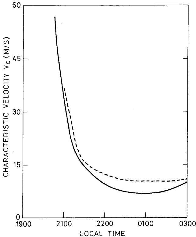
Fig. 14. Variation of measured characteristic velocity ( V_c ) with local time (solid line) and estimate of the variation of \sigma_e with local time (dotted line) (Bhattacharyya et al. , 1989).
