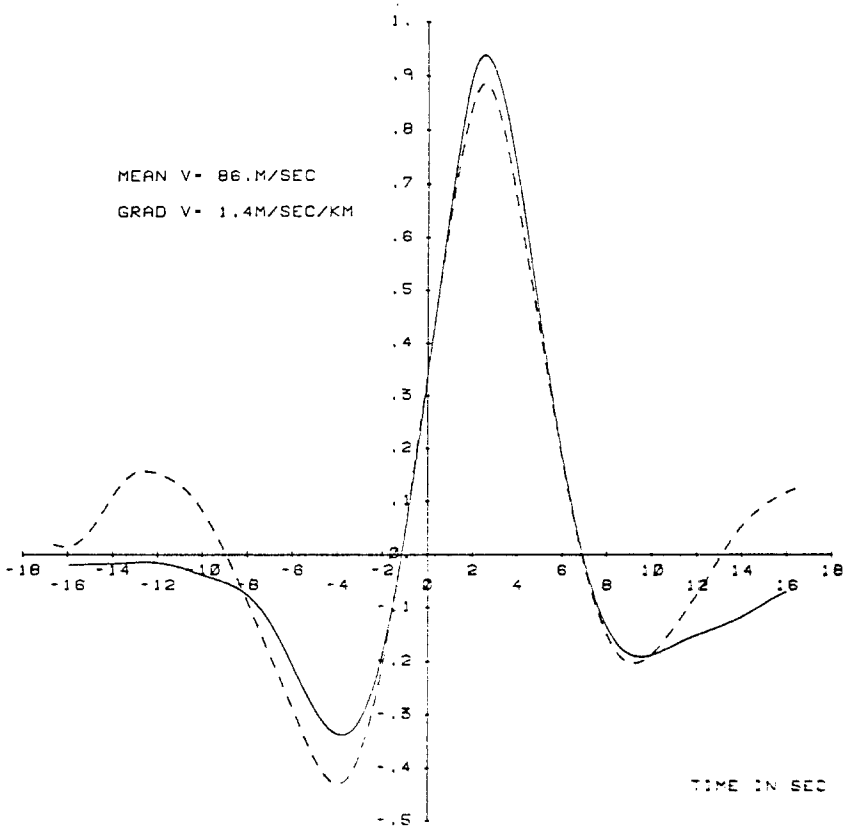
Fig. 11. (a) Comparison between the measured (dashed line) and modeled (solid line) correlation function for receivers separated by 244 m. In the model, the irregularity drift velocity is taken to vary linearly along the propagation path. (b) Same as (a) for cross-correlation functions (Wernik et al. , 1983).
