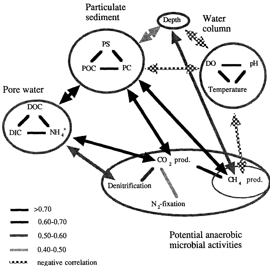
Fig. 4. Schematic representation of the significant Pearson correlations among the physical, chemical, and microbial variables measured from June to September 1990.
