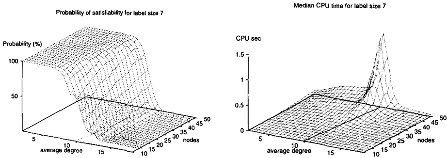
Figure 3. Probability of satisfiability and median CPU time for A(n, d, 7.0) .
