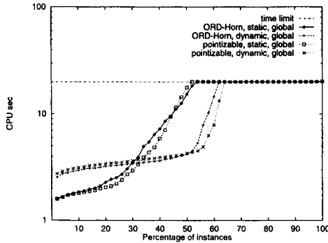
Figure 9. Runtime performance on S(100, 25, 6.5) (500 instances overall).
