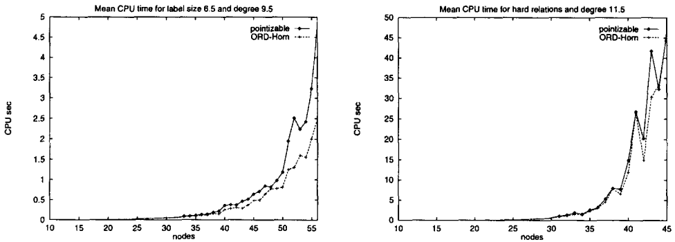
Figure 5. Comparison between \mathcal{P} and \mathcal{H} for A(n, 9.5, 6.5) and H(n, 11.5) (500 instances per data point).
