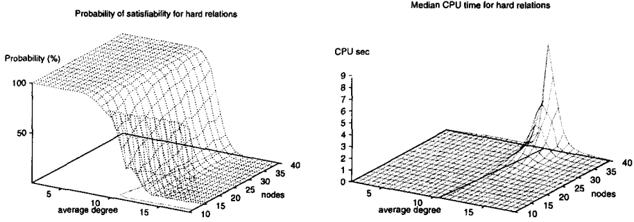
Figure 4. Probability of satisfiability and median CPU time for H(n, d) (500 instances per data point).
