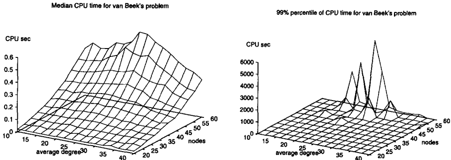
Figure 8. 50% and 99% percentile of CPU time on S(n, d, 6.5) (500 instances per data point).
