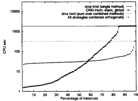
Figure 10. The effect of combining strategies orthogonally (500 instances overall).
