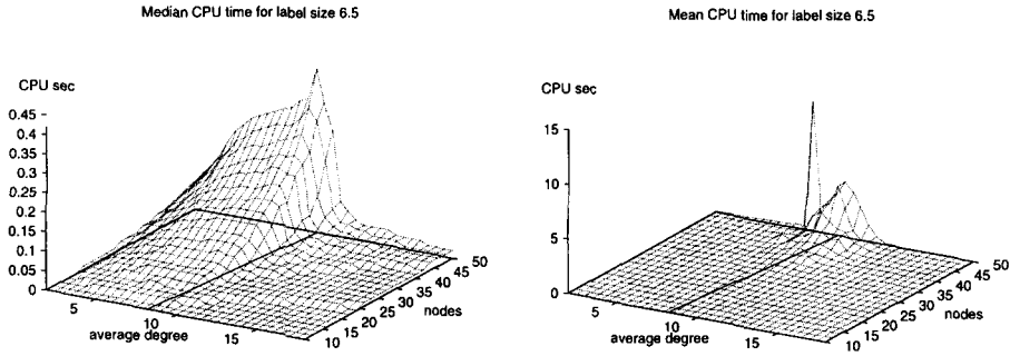
Figure 2. CPU time for A(n, d, 6.5) (500 instances per data point).
