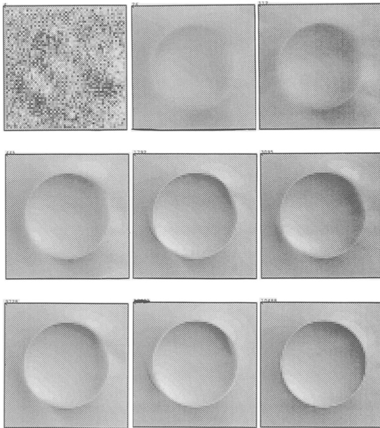
Fig. 7. Reconstruction of a crater-like shape. Points on the rim in the northeast and the southwest correspond to places in the input image where there is least contrast between the inside and the outside, since the direction of the incident illumination is parallel to the rim there.
