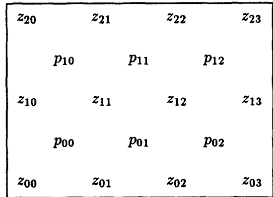
Fig. 3. It is convenient to have the discrete grid for p , q (and hence for the image E itself) offset by 1/2 picture cell in x and 1/2 picture cell in y from the grid for z .
