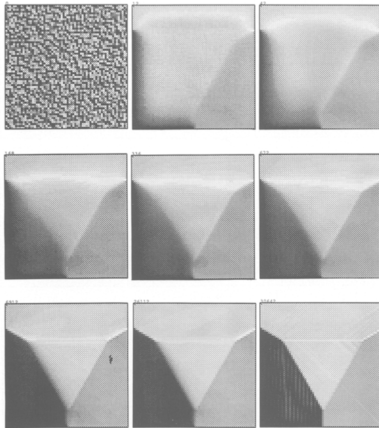
Fig. 6. Reconstruction of a portion of a truncated hexahedron from a shaded image. The dihedral angle between each pair of the three outer surfaces is \pi/2 . This example illustrates the algorithm's ability to deal with surfaces that have large discontinuities in surface orientation.
