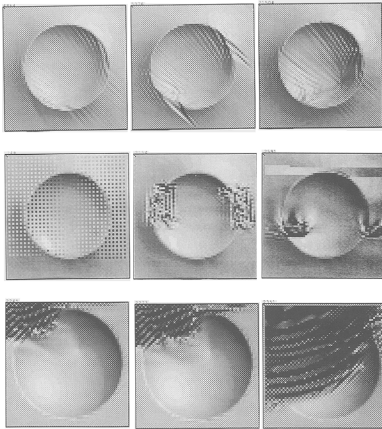
Fig. 11. Graphical depiction of instabilities and the effects of programming errors. In the top row are shown instabilities resulting from too rapid reduction of the penalty term for departure from smoothness. The middle row shows the results of various programming errors. The bottom row shows waves of instability propagating inwards from a free boundary.
