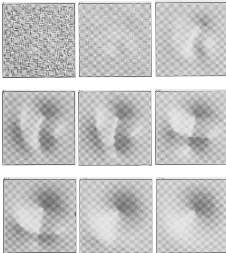
Fig. 10. What happens when the algorithm is confronted with an impossible shaded image? The input image here (not shown) is a circularly symmetric dark smudge in a uniformly bright surround. The light source is assumed to be near the viewer. The algorithm finds a “solution” with a single conical singularity.
