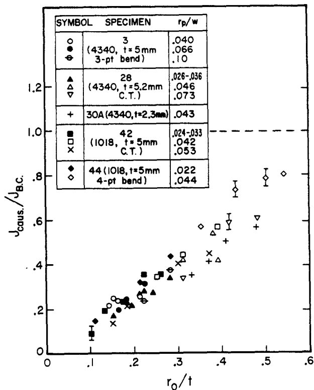
Figure 4. J_{caus.}/J_{BC.} vs. r_0/t . Deviation from unity indicates three dimensional field for r/t < 0.6 or 0.7 .
