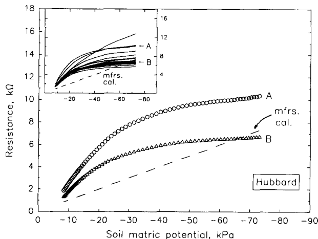
Fig. 3. Block resistance versus soil matric potential data for the two blocks (A and B) in Hubbard loamy sand. The dashed line represents the calibration provided by the manufacturer. The inset shows calibration curves for all 20 blocks.
