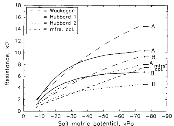
Fig. 4. Calibration curves for soil matric potential for the same two blocks (A and B) in Waukegan silt loam and Hubbard loamy sand. Hubbard 1 and 2 represent duplicate calibrations.
