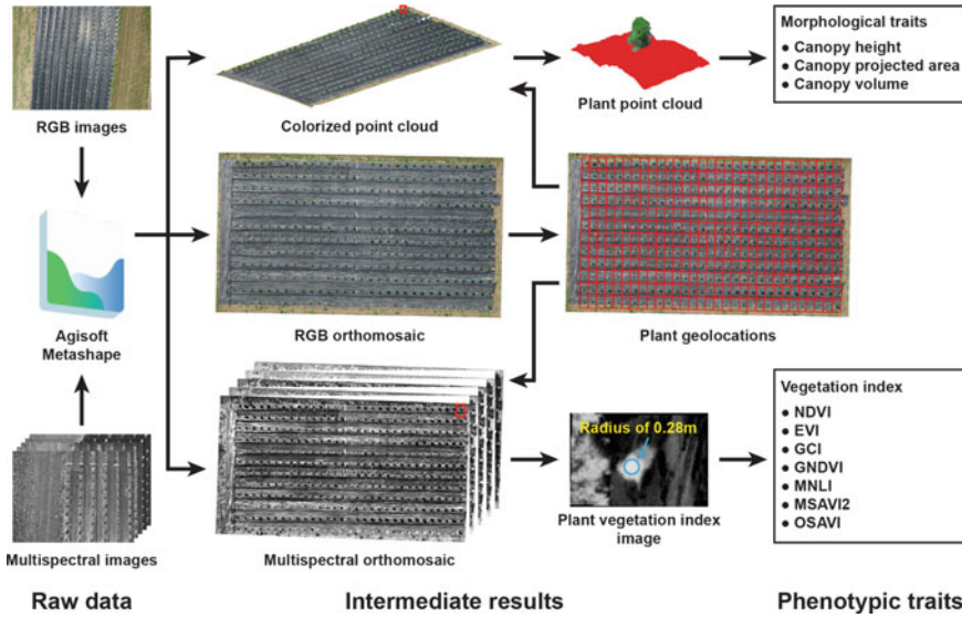
Fig. 2.7 Data processing pipeline for the extraction of phenotypic traits from RGB and multispectral data. Derived vegetation indices include normalized difference vegetation index (NDVI), enhanced vegetation index (EVI), green chlorophyll index (GCI), green normalized difference vegetation index (GNDVI), modified non-linear index (MNLI), modified soil adjusted vegetation index 2 (MSAVI2), and optimized soil adjusted vegetation index (OSAVI)
