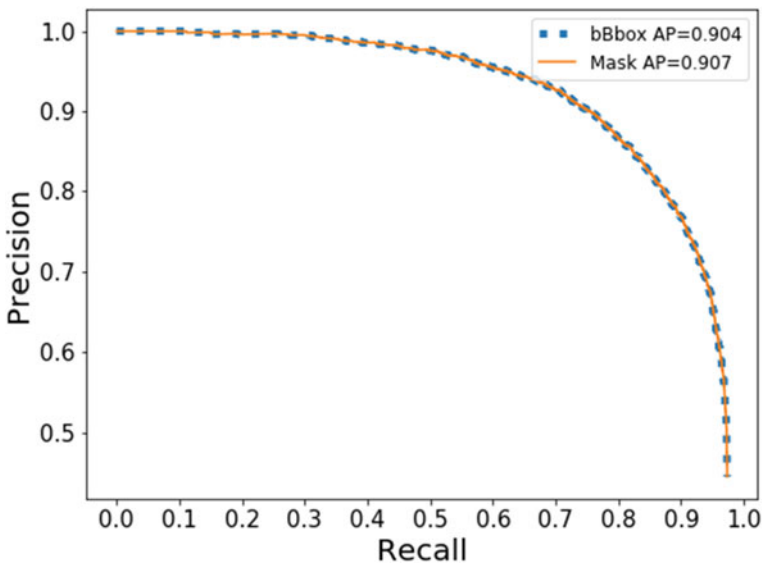
Fig. 6.7 The curve of precision and recall
