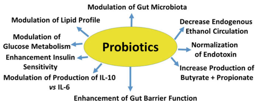
Fig. 5.3 Possible mechanisms of bio-therapeutic effects of probiotics against NAFLD
