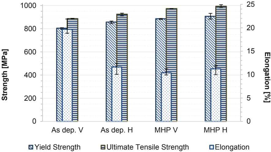
Fig. 6. Tensile properties of as deposited and inter-pass MHP of thin walls
