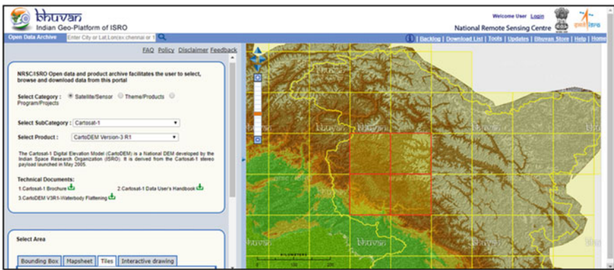
Fig. 23.8 Bhuvan portal showing CartoDEM tiles highlighted (red color) over Srinagar, Jammu, and Kashmir for downloading
