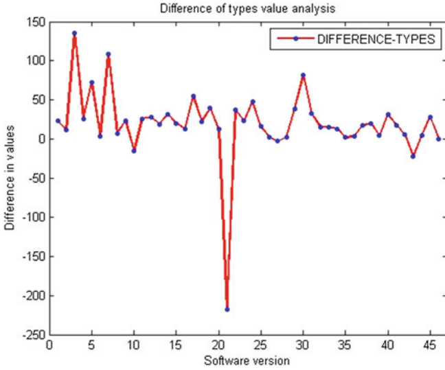
Fig. 8 Difference of types values analysis
