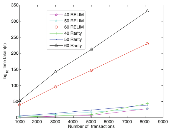
Fig. 3 Number of transactions versus log time taken for mushroom
