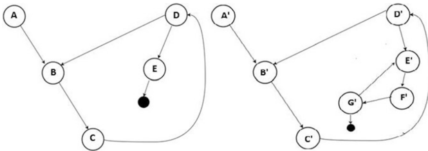
Fig. 6 Optimized CFGs G and G' of the original and the obfuscated program
