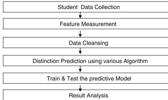
Fig. 1 Methodology used
