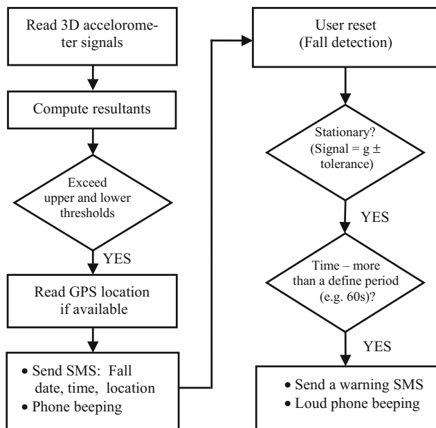
Fig. 1 A block diagram showing the fall detection algorithm
