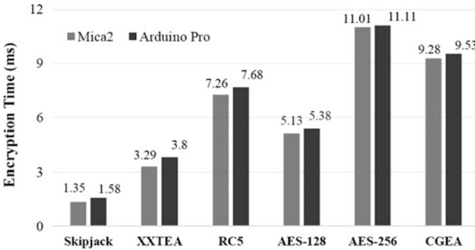
Fig. 2 Encryption time
