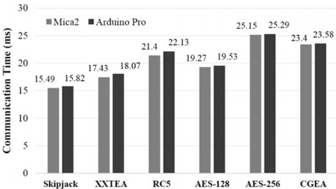
Fig. 3 Communication time
