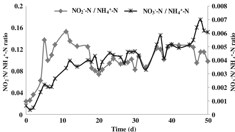
Fig. 10 Molar ratio during landfill leachate treatment in AnMBR. Source Suneethi and Joseph (2013)
