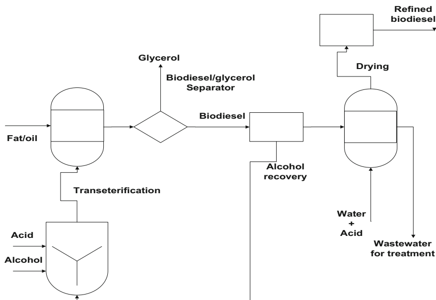
Fig. 1 Conventional process flow of biodiesel production (Daud et al. 2015)
