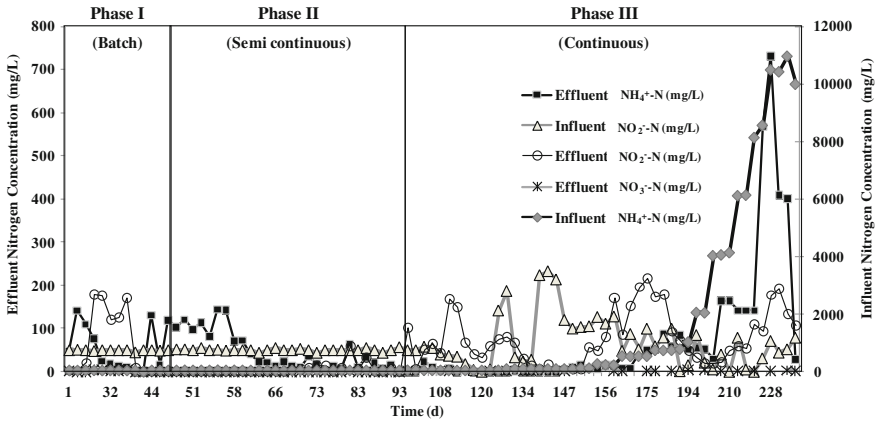
Fig. 8 Nitrogen transformations at varying nitrogen loading rates in the AnMBR. Source Suneethi and Joseph (2011b)
