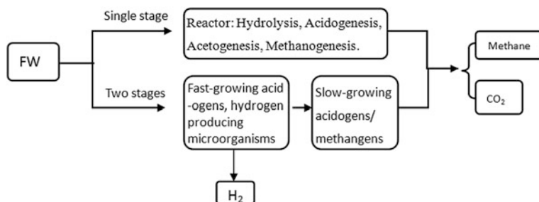
Fig. 4 The process flow of methane production from FW
