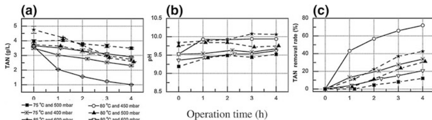
Fig. 13 Ammonia stripping experiment a TAN concentration, b pH of liquid sample and c accumulated TAN removal rate at different operation (Nie et al. 2015)
