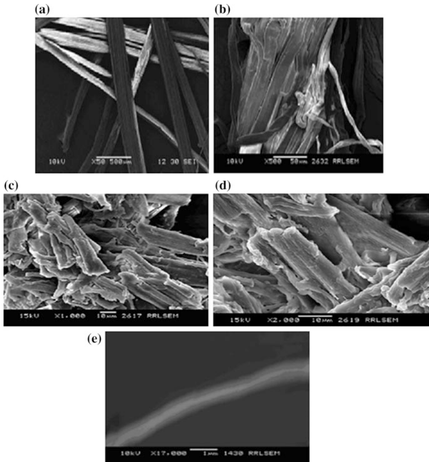
Fig. 6.26 SEM photographs of different banana fibers. a is untreated banana fiber ( \times 50 ); b is banana fiber treated by steam explosion ( \times 500 ); c is banana fiber by bleaching ( \times 1000 ); d is banana fiber by bleaching ( \times 2000 ); e is banana fiber by bleaching acid ( \times 17,000 )
