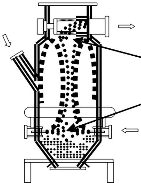
Fig. 6.38 Pulverizer of biomass
