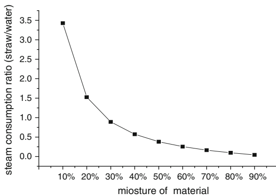
Fig. 2.20 Effect of material moisture content on the ratio of heating materials energy to heating the liquid water in materials energy. Prerequisite: 20\text{-m}^3 tank, inlet steam temperature 220 \text{ }^\circ\text{C} , heating the material from room temperature 20\text{--}182 \text{ }^\circ\text{C} , and holding time 5 min
