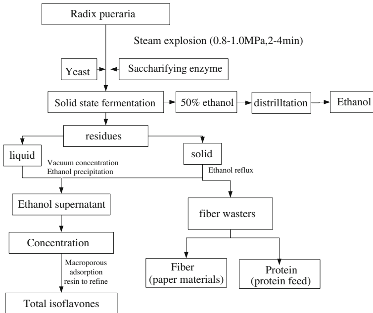
Fig. 6.17 Production of ethanol and isoflavones from steam pretreated Radix Pueraria by solid-state fermentation
