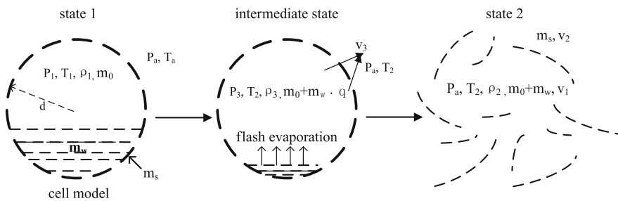
Fig. 2.4 Simple model for steam explosion at the cellular level
