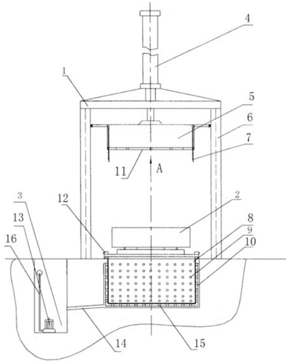
Fig. 3.20 Press-type dehydration equipment. 1, 6 Rack; 2 material; 3 sump; 4 hydraulic cylinder; 5 squeeze plate; 7 steel chain; 8 U-shaped steel mold; 9 drainage holes; 10 groove; 11, 15 drain groove; 12 hook; 13 pump; 14 input pipe; 16 output pipe
