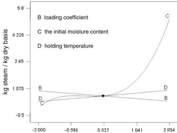
Fig. 2.18 Single factor response curve to steam consumption per unit mass of dry basis (kg steam/kg dry basis)
