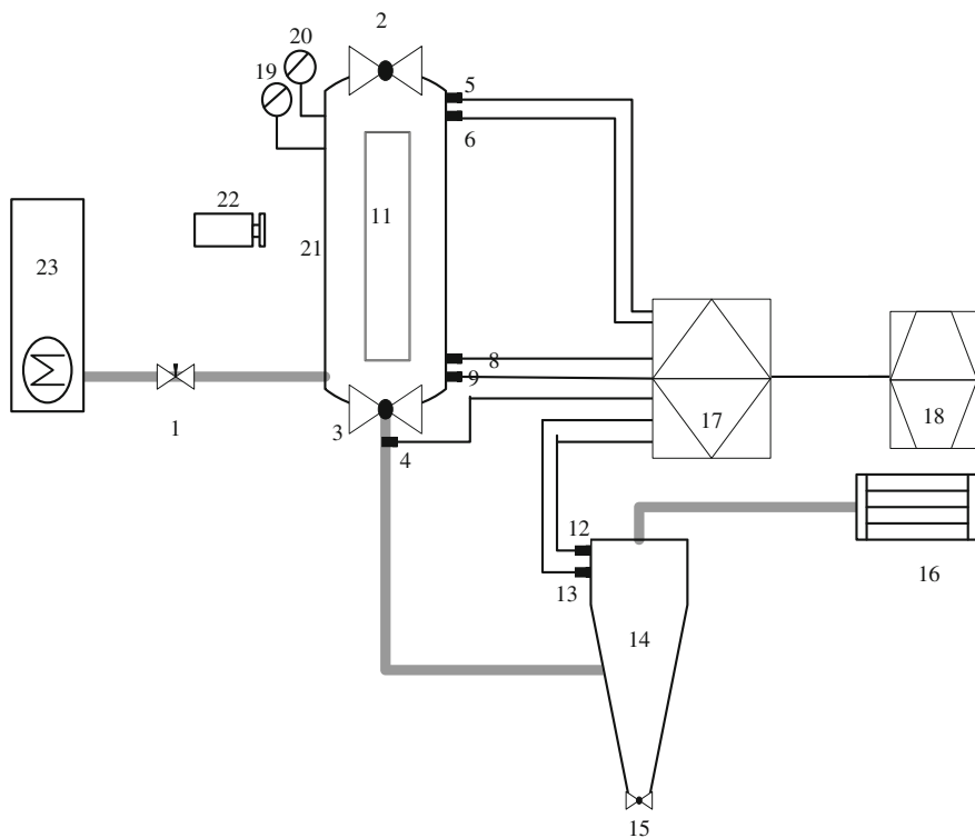
Fig. 1.1 Laboratory gas explosion apparatus
