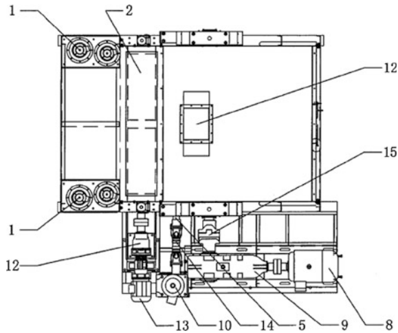
Fig. 3.12 Aerial view of straw baler losing machine. 1 Feed roller; 2 upper roll; 3 transitional roller; 4 package material roller 1; 5 package material roller 2; 6 cover; 7 rack; 8 motor 1; 9 reduction drive; 10 motor 2; 11 conveyor; 12 drive motor 1; 13 drive motor 2; 14 Cardan joint; 15 cross-linked coupling
