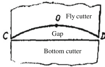
Fig. 3.1 Fly cutter, bottom cutter, and gap of knife-roll straw cutter
