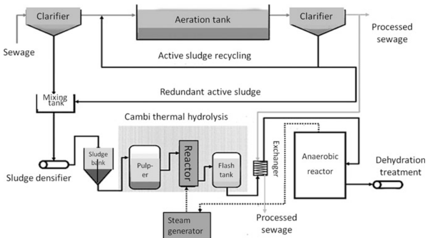
Fig. 6.20 Cambi gas explosion processes [57, 58]
