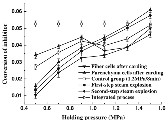
Fig. 4.9 Effects of the steam explosion and mechanical carding methods on the inhibitor content
