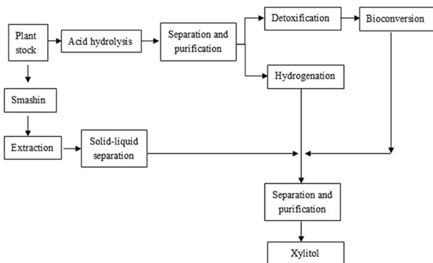
Fig. 6.40 Traditional preparation technology of xylitol [94]
