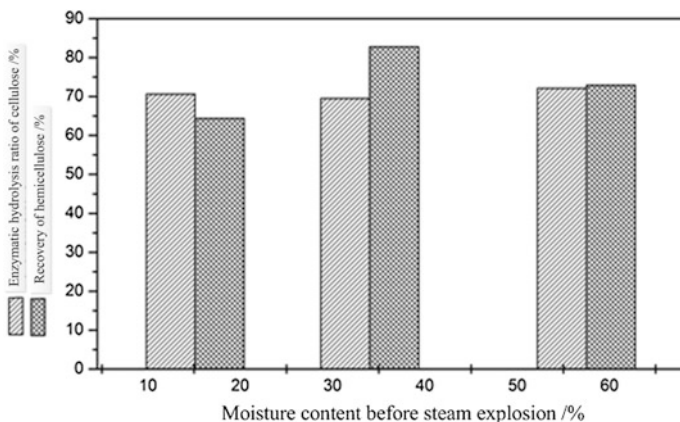
Fig. 4.7 Effects of moisture on the steam explosion performance (1.5 MPa, 10 min)
