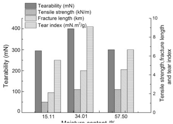
Fig. 2.3 Effect of the initial moisture content of materials on property of pulp (1.5 Mpa, 10 min) [1]
