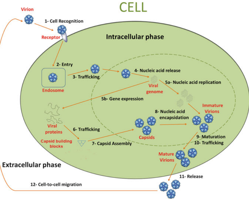
Fig. 1.4 A generic viral cycle. The following stages of the cycle are schematized: 1 Recognition of host cell receptor(s) on the host cell surface. 2 Entry of the virus particle (or of some components) into the host cell. 3 Trafficking of the viral particle (or some components) in the host cell. 4 Release of the nucleic acid. 5a Replication of the viral genome. 5b Expression of the viral genome. 6 Trafficking of the synthesized virus components to sites where the morphogenesis of virus particles will take place. 7 Assembly of the virus capsid from the previously synthesized CP subunits. 8 Packaging of the nucleic acid genome inside an assembled capsid (capsid assembly and nucleic acid packaging may occur concomitantly). 9 Maturation of the virus particle. Depending on the animal virus species, stages 4, 5a, 5b (in part), 6, 7, 8 and 9 may occur in either the cytoplasm or the nucleus of the host cell; this is indicated in the figure by encircling those steps by a discontinuous line, which represents the nuclear membrane only in those cases where the processes indicated occur in the cell nucleus. 10 Intracellular trafficking of the virus particles and/or mature virions, which may occur between, during and/or after steps 7, 8, and/or 9. 11 Release of virions from the cell. 12 Navigation of virus particles in the extracellular environment. See text for a more complete description and some important variations (Figure kindly provided by M.A. Fuentes)
