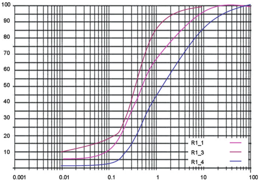
Fig. 18.5 Location of samples and results presented with cumulative curves of deposits in key site R1
