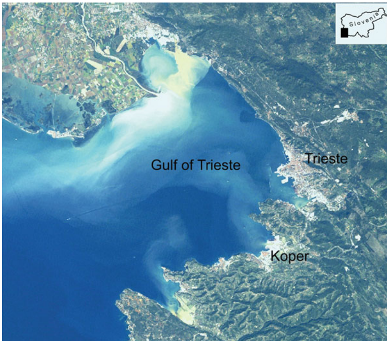
Fig. 8.8 Sediments from floodwaters visible in the Gulf of Trieste (in the northern Adriatic) (© NASA Landsat TM5, 21 September 2010)
