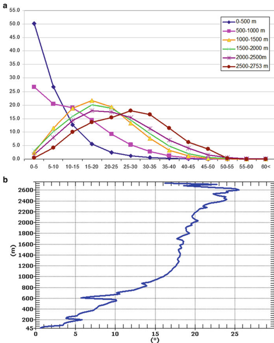
Fig. 17.1 Elevation/slope plots of elevation zones of 500 m interval in percentage (a); mean slope plotted against elevation (b)
