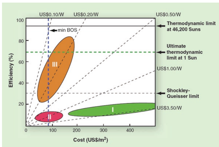
Fig. 4 Photovoltaic (PV) power costs ($/W) as function of module efficiency and areal cost. The cost figure of merit for PV cell modules ($/W) is determined by the ratio of the module cost per unit area divided by the maximum electric power per unit area. Dashed lines are constant $/W. Highlighted regions refer to Generation I, Generation II ( thin-film PV ), and Generation III (advanced/future PV) solar cells (From Green [6])
