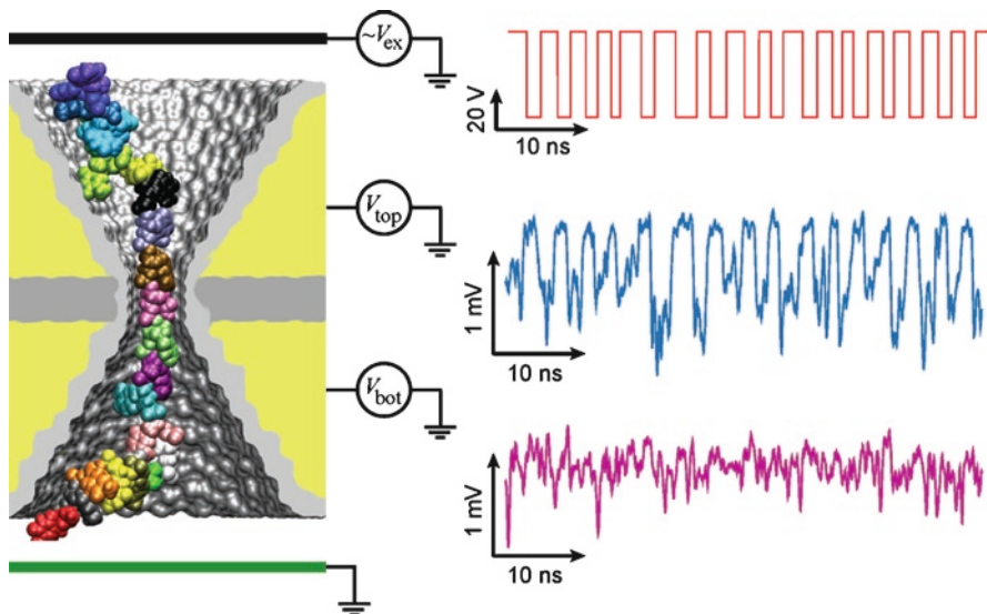
Fig. 8 Driven by an external electric field, a DNA molecule permeates a nanometer-size pore in a multilayer semiconductor membrane. The nucleotide sequence of the DNA molecule is recorded as the change of the electrostatic potential in the capacitor (From Sigalov et al. [54])
