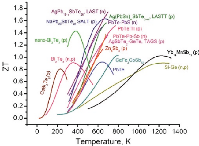
Fig. 13 Current state of the art in bulk thermoelectric materials. All the top performing (high ZT ) materials are nanostructured. ZT \geq 3 is needed for many practical applications of thermoelectrics [36]
