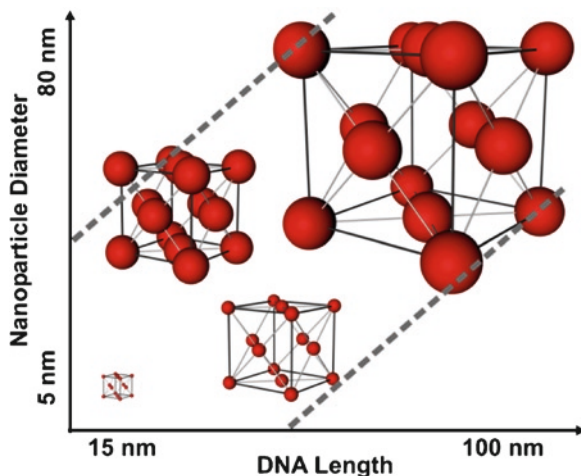
Fig. 13 Illustration of the “zone of crystallization” (denoted by dashed lines ) in which certain combinations of nanoparticle size and DNA length are able to form ordered superlattices. Modeled unit cells are drawn to scale relative to one another [57]
