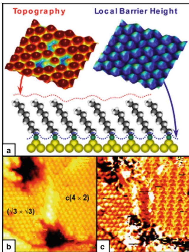
Fig. 2 Simultaneous STM measurements yield absolute tilt angles of individual molecules in self-assembled monolayers [17]
