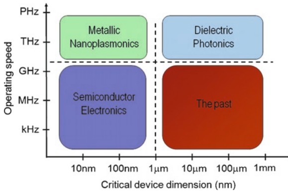
Fig. 7 Graph of the operating speeds and critical dimensions of different chip-scale device technologies. Different domains in terms of operating speed and device sizes are expected to heavily rely on the unique material properties of semiconductors (electronics), insulators (photonics), and metals (plasmonics). The dashed lines indicate physical limitations of different technologies; semiconductor electronics is limited in speed by interconnect delay time issues to about 10 GHz. Dielectric photonics is limited in size by the fundamental laws of diffraction. Plasmonics can serve as a bridge between similar-speed dielectric photonics and similar-size nano-electronics (Adapted from Brongersma and Shalaev [3])
