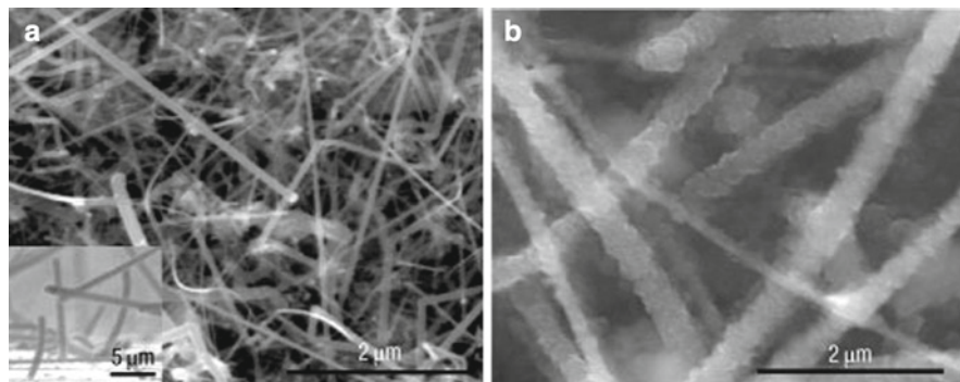
Fig. 5 Nanostructured materials, such as these Si nanowires used as an anode in a Li ion battery before (a) and after (b) electrochemical cycling (From Chan et al. [10]) have the potential to increase the performance of batteries by ten times or more
