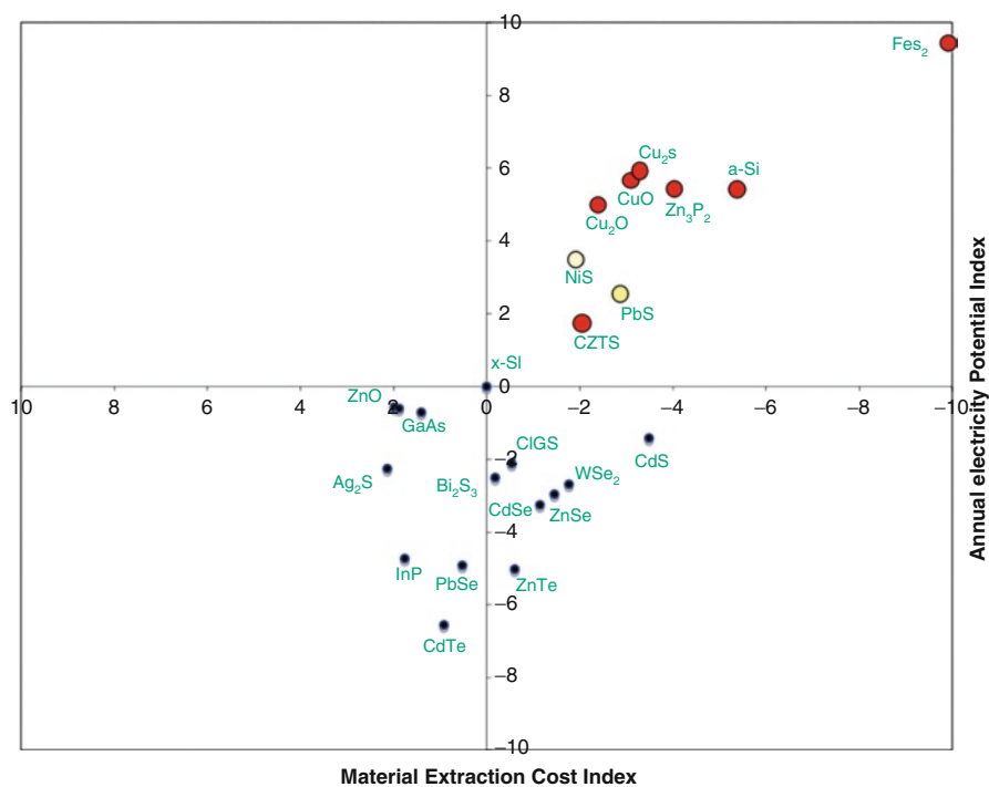
Fig. 10 Various inorganic materials ranked by extraction costs and electricity production potential for photovoltaic applications from the paper by Wadia et al. [16] Materials in red are those the authors identified with the greatest long-term potential. Nanotechnology to enhance light absorption, facilitate thin-film processing, improve the ratio of carrier collection to recombination loss, and tune bandgaps could be beneficial for many materials combinations
