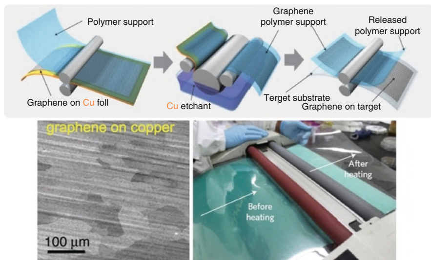
Fig. 16 Images of large scale production of graphene grown on copper foils and transferred to a polymer layer for use in large area display applications (From Li et al. [61] and Bae et al. [62])
