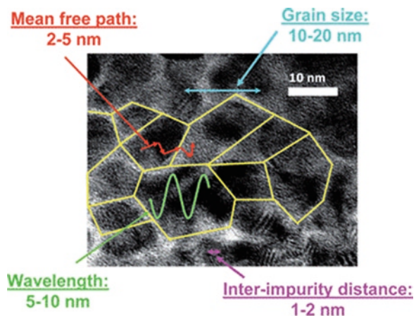
Fig. 7 A TEM image of a heavily doped \text{Si}^{80}\text{Ge}^{20} nanocomposite along with some important numerically calculated characteristic lengths [19]
