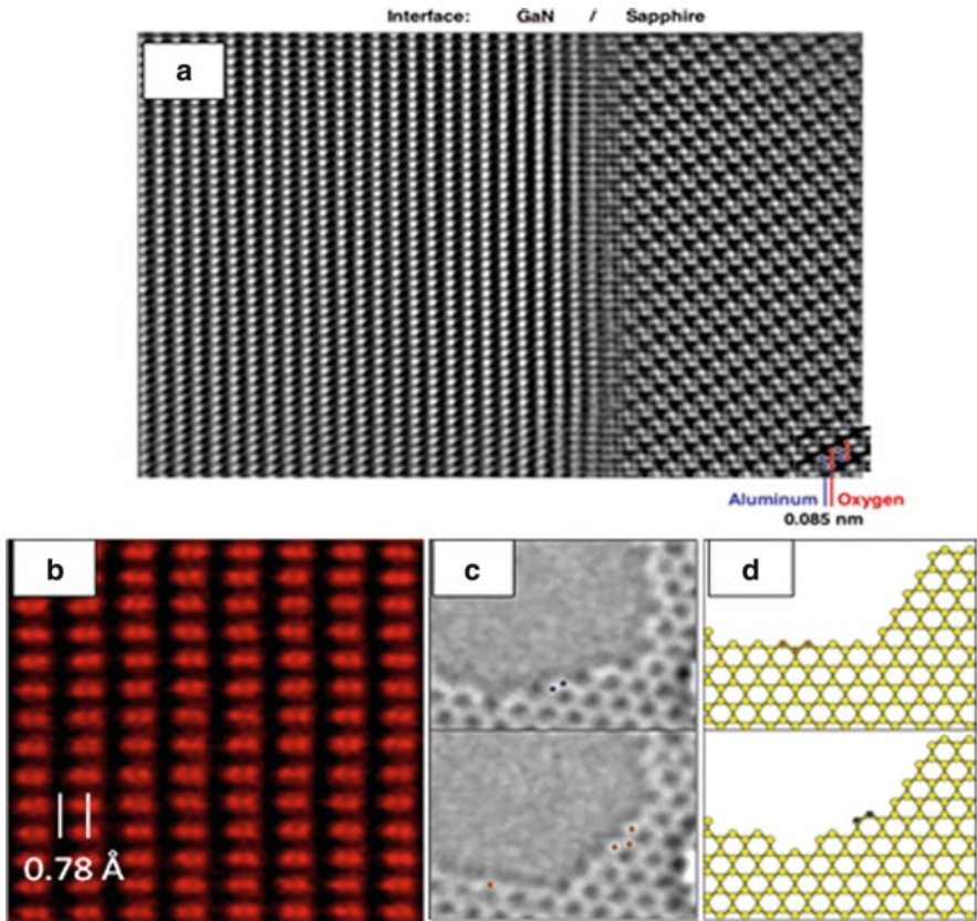
Fig. 5 Montage of atomic-scale images and phenomena enabled by aberration-corrected S/TEM. (a) HREM image of an interface between GaN and sapphire (Courtesy of Lawrence Berkeley National Lab.); (b) Silicon “dumbbells” at sub-Ångstrom resolution via HAADF/STEM (Courtesy of O. Krivanek, NION Corp. and S. Pennycook, Oak Ridge National Lab.); (c) Dynamics of graphene with atom-by-atom motion in successive frames. Right side illustrations show schematics of the process. (Courtesy of A. Zettl and C. Kisielowski, from Girit et al. [34])
