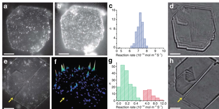
Fig. 4 Wide field images of catalytic reactions on individual LDH particles. Transesterification of C-FDA with 1-butanol at 40 nM (a) and 700 nM (b) ester concentration on the same LDH crystal. (c) Distribution of initial reaction rates for 1 \mu\text{m}^2 domains on the crystal faces ( n=50 ). (d) Transmission image of the crystal. (e-h) Hydrolysis of 600 nM C-FDA on LDH crystal. (e) Fluorescence image, showing formation of single product molecules mainly at crystal edges (96 ms per image). (f) Accumulated spot intensity on the same crystal over 256 consecutive images. (g) Distribution of initial reaction rates for 1 \mu\text{m}^2 domains on the faces of the LDH crystal ( n=207 ). The distribution clearly shows two statistically different subpopulations. The fast population corresponds to active domains located on the \{1010\} faces (right graph), whereas the \{0001\} faces host the slow population (left graph). (h) Transmission image. Scale bars, 5 \mu\text{m} . Arrows in e, f, h indicate the same viewing direction on the same crystal [25]
