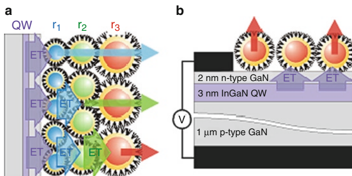
Fig. 12 (a) Schematic of a potential white light emitter: nanocrystals with emission at 480 nm ( r_1 ), 540 nm ( r_2 ), and 630 nm ( r_3 ). (b) Schematic of an electrically driven, single-color energy transfer device (Adapted from Achermann et al. [53])
