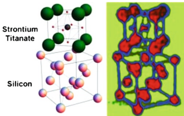
Fig. 22 (Left) The arrangement between atoms of a film of strontium titanate and single crystal of silicon on which it was made. When sufficiently thin, strontium titanate can be strained to match the atom spacing of the underlying silicon and becomes ferroelectric. (Right) The schematic at the left has been written into such a film using the ability of a ferroelectric to store data in the form of a reorientable electric polarization (Courtesy of J. Levy, University of Pittsburgh)
