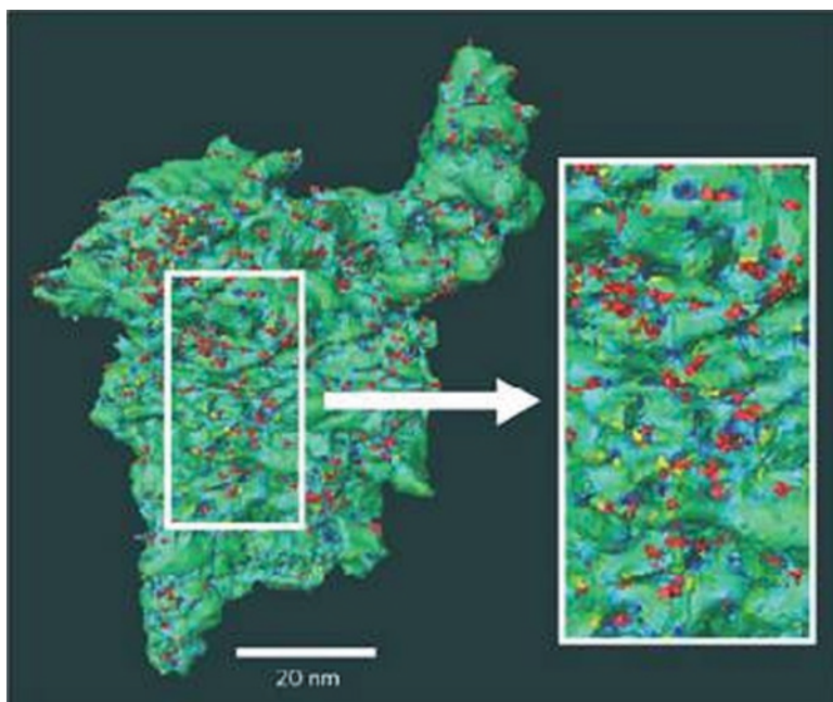
Fig. 16 3D tomographic reconstruction of a heterogeneous catalyst based on disordered mesoporous silica supporting bimetallic ruthenium–platinum nanoparticles [91]
