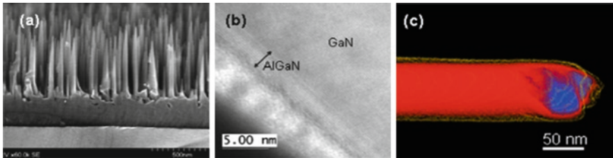
Fig. 11 Images of nanowires with approximately 2.5-nm thick AlN or AlGaIn shell layers surrounding GaN cores. (a) SEM image, (b) high-resolution cross-section TEM image, and (c) reconstructed 3D scanning TEM tomograph showing AlN at edges, GaN core, and embedded Ni catalyst at the tip [50, 51]
