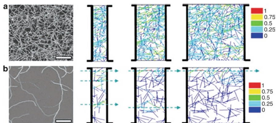
Fig. 2 SEM images ( left ) and simulated normalized current distribution for carbon nanotube networks with high ( a ) and low ( b ) coverage. Measurements were reported on SWNTs grown by chemical vapor deposition with systematically varying degrees of alignment and coverage in transistors with a range of channel lengths and orientations perpendicular and parallel to the direction of alignment. A stick-percolation-based transport model provides a simple yet quantitative framework to interpret the sometimes-counterintuitive transport measured in the devices that cannot be reproduced by classical transport models (After Kocabas et al. [32])
