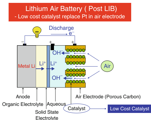
Fig. 14 Organic and aqueous electrolytes, separated by a solid state electrolyte, are used to create a new lithium-air battery, resulting in a large capacity (50,000 mAh/g on air electrode basis) [83]
