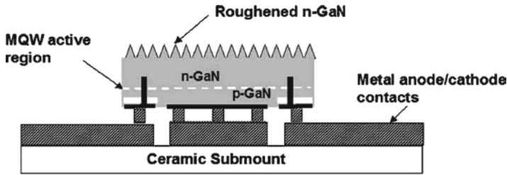
Fig. 6 State-of-the-art thin-film flip-chip (TFFC) InGaN-GaN light-emitting diode
