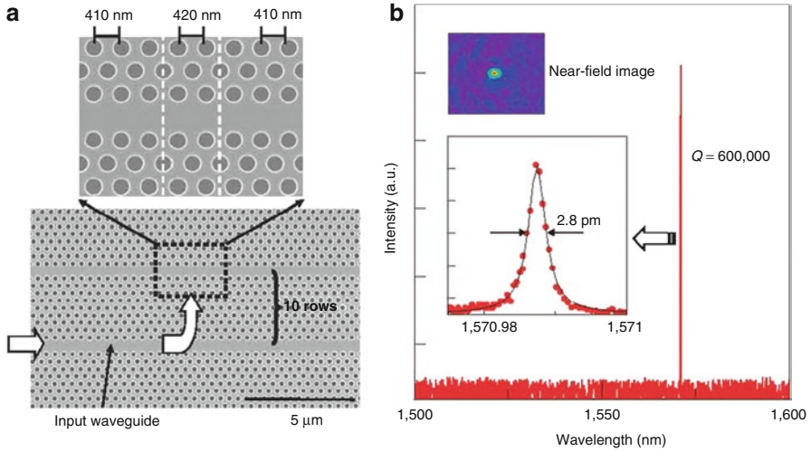
Fig. 1 (a) SEM of fabricated photonic crystal structure. (b) spectrum of the cavity, showing Q = 600,000 [12]
