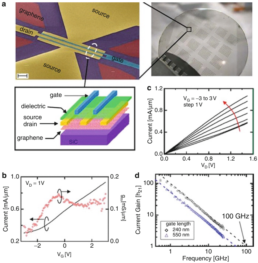
Fig. 2 (a) Scanning electron microscope image and the schematic cross-sectional view of a top-gated graphene field-effect transistor. The optical image of the 2 in. graphene/SiC wafer with arrays of graphene devices is on the right. The transistors possess dual-gate channels to increase the drive current and lower the gate resistance. The scale bar is 2 μm. (b) Drain current I_D of a 240 nm gate length graphene transistor as a function of gate voltage V_G at drain bias of 1 V. The current shown was normalized with respect to the total channel width. The device conductance g_m = dI_D/dV_G is shown on the right axis. (c) Measured drain current I_D as a function of drain bias of a graphene FET with a gate length L_g of 240 nm for various top-gate voltages. (d) Measured small signal current gain |h_{21}| as a function of frequency f for a 240 nm gate and a 550 nm gate graphene FET, represented by (\diamond) and (\Delta) , respectively. The current gain for both devices exhibits 1/f dependence, where a well-defined cutoff frequency f_T can be determined to be 53 GHz and 100 GHz for the 550 nm and 240 nm devices, respectively [57]
