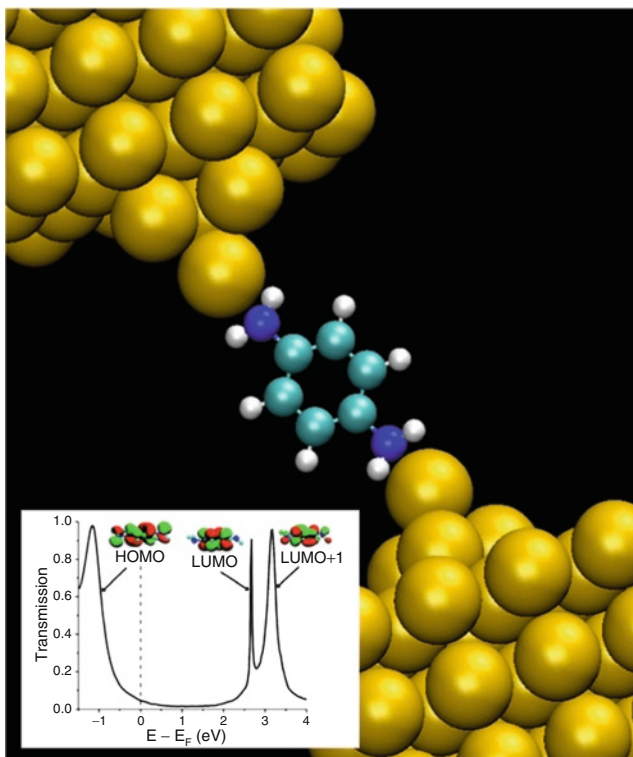
Fig. 1 First-principles density functional theory (NEGF-DFT) simulations of the conductance of molecular junctions have led to improved understanding and quantitative agreement with experiments. The figure shows the calculated atomic geometry of benzene-diamine suspended between Au electrodes; the inset shows the computed electron transmission vs. energy [5]
