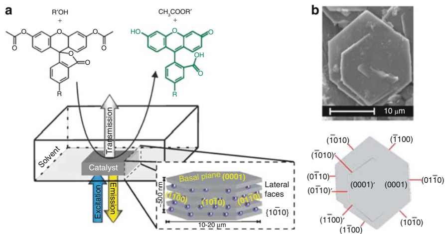
Fig. 3 Experimental set-up. (a) Schematic drawing of the experimental set-up: the LDH particle is exposed to fluorescein ester ( R = -\text{COOH} for C-FDA; R = -\text{H} for FDA) in R'\text{OH} solution ( R' = -\text{H} for hydrolysis; R' = -n\text{C}_3\text{H}_9 for transesterification). A wide field microscope with 488 nm excitation light was used. The inset shows the different crystallographic faces of a hexagonal LDH crystallite with indication of the Miller indices. (b) Scanning electron micrograph of a typical LDH crystal with assignment of the different crystal faces for the intergrown crystal (From Roeffaers et al. [25])
