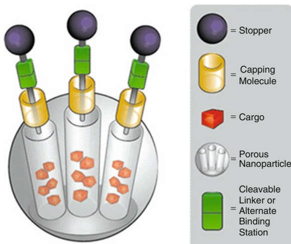
Fig. 17 Graphical representation of a mesoporous silica nanoparticle ( \text{SiO}_2 , average diameter of 200 nm) adorned with a layer of [2] rotaxanes on the nanoparticle surface. Cargo can be released from the pores of the nanoparticles by either forcing the capping molecule to move to another binding site of the rotaxane stalk (nanovalves), or by cleaving the rotaxane stoppers off the stalks completely (snap-tops) (Courtesy of F. Stoddart and A. Nel)
