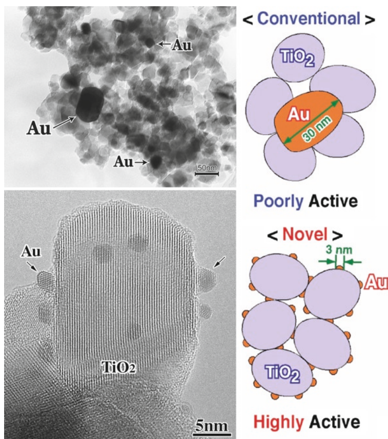
Fig. 6 Comparison of the nanostructure of poorly active and highly active Au-based catalysts (Courtesy of M. Haruta)
