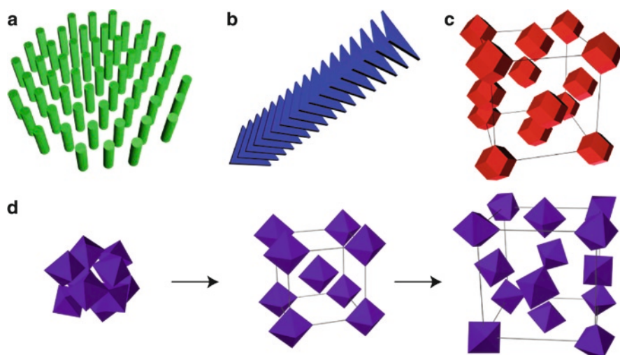
Fig. 14 Models of superlattices derived from DNA-mediated assembly of anisotropic nanostructures. (a) 2D hexagonal arrangement of nanorods. (b) 1D columnar ordering of triangular nanoprisms. (c) Face-centered cubic ordering of rhombic dodecahedra. (d) Illustration of the transition from disordered to BCC to FCC ordering with increasing linker length in the assembly of octahedra [58]
