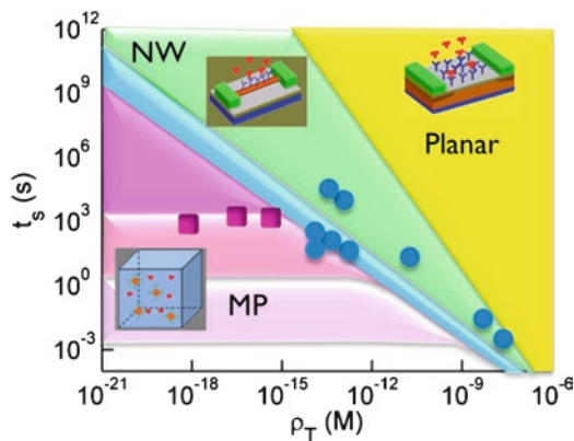
Fig. 11 Phase space of biosensor response. The different regions show the analyte concentration ( \rho_T ) that can be measured in a given sampling time ( t_s ). Classical planar sensors require more time to detect a given analyte concentration. Planar, nanowire (NW), and magnetic particle (MP) sensors behave differently due to their different diffusion characteristics. The enhanced sensitivity of MP bio-barcode sensors is due to a reduction of the diffusion bottleneck by dispersing the “sensors” with the volume of the analyte. (Symbols denote sources of experimental data: NW (dots) from Zheng et al. [64], Gao et al. [61], Stern et al. [63], Kusnezow et al. [62], Li et al. [19]; MP (squares) from Goluch et al. [65], Nam et al. [66], and Nam et al. [67])
