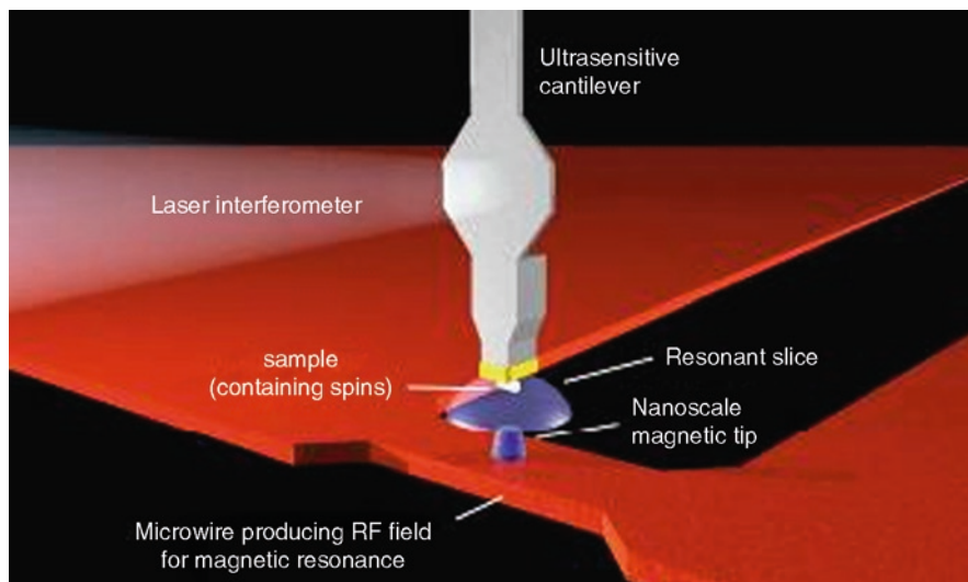
Fig. 13 Schematic diagram of magnetic resonance force microscopy (From Degen et al. [60])
