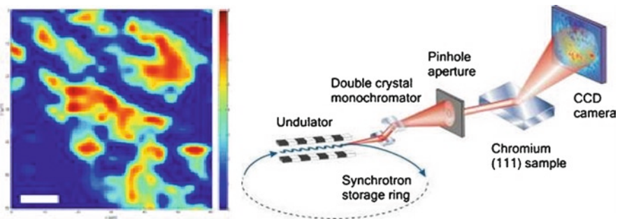
Fig. 8 Diagram of the experimental set-up and charge-coupled device (CCD) image of the x-ray speckle observed for the [200] lattice Bragg reflection
