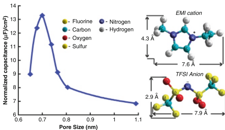
Fig. 20 Normalized capacitance change versus the pore size of the carbide-derived carbon samples tested in an ionic liquid electrolyte. Normalized capacitance is obtained by dividing the gravimetric capacitance by the specific surface area. HyperChem models of the structure of ethyl-methylimidazolium (EMI) and bis(trifluoro-methane-sulfonyl)imide (TFSI) ions show a size correlation [77]
