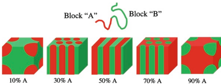
Fig. 3 Some key periodic nanostructure phases produced naturally by diblock copolymers as controlled by block volume fraction (Courtesy of M. Tuominen)
