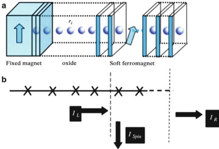
Fig. 9 (a) Schematic of an STT device. An insulator is sandwiched between two ferromagnets. The magnetization of the fixed magnet is kept unchanged. On the other hand, the magnetization of the soft ferromagnet can be changed by applying a spin polarized current through it. (b) A simple depiction of underlying physical mechanism. The difference between the spin angular momentum at the left and right interfaces of the soft ferromagnet is absorbed by the magnet itself. This subsequently tries to realign the magnetic orientation to the direction of polarized spins (From Salahuddin et al. [56])
