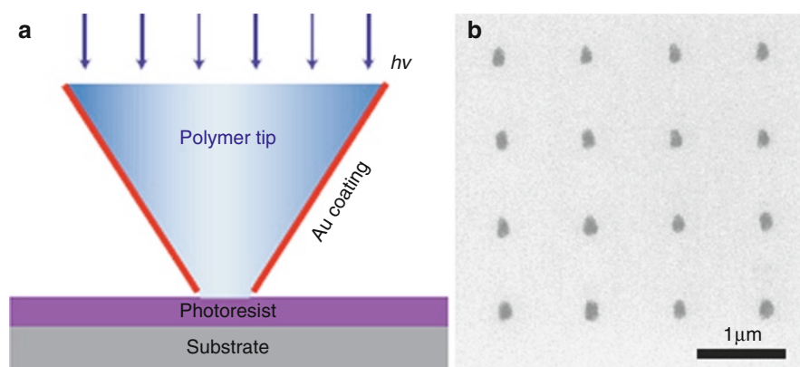
Fig. 8 (a) Scheme of beam pen lithography. (b) Scanning electron micrograph of 100 nm features made using 400 nm light [43]
