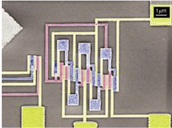
Fig. 7 Implementation of a CMOS-type 5-stage ring oscillator on a single carbon nanotube [90]
