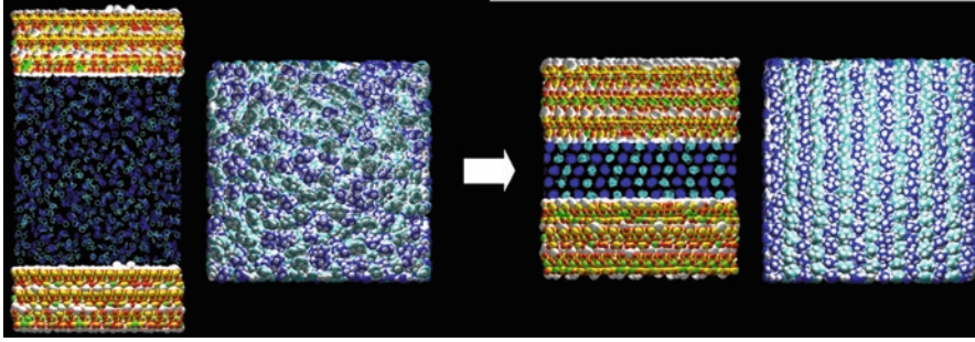
Fig. 12 Upon sufficient nanoconfinement, cyclohexane undergoes a rapid and abrupt transition to a layered and hexagonal ordered, solid-like structure. In the configurations, the mica sheets are shown and the cyclohexane rendered in stick form on the left, so that it is easy to see through the confined fluid; the confined fluid, rendered in full size without mica, is shown on the right , looking down from above. Cyclohexane molecules (H atoms white , C atoms shades of blue ) are colored in two different shades of gray , making the resulting order apparent (From Docherty and Cummings [71])
