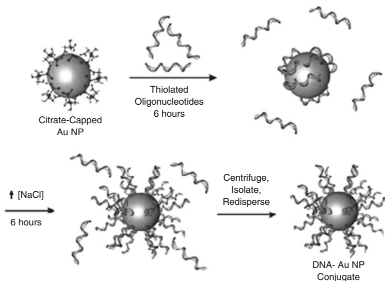
Fig. 5 Synthesis of DNA AuNPs. Citrate-capped gold nanoparticles are mixed with alkyl-thiol modified oligonucleotides for 6 h. The thiol adsorbs to the AuNP surface resulting in a loose association of DNA with the particle surface. Through a process of salt (NaCl) additions, the particles are ‘aged’ over 6 h to achieve a dense loading of alkyl-thiol oligonucleotides to the surface of the AuNP. Centrifugation isolates the DNA AuNP conjugates from unreacted components (Courtesy of Chad Mirkin)
