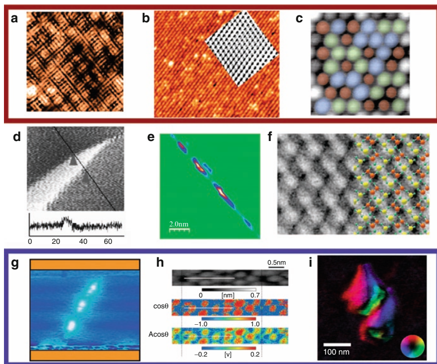
Fig. 1 Spatially resolved properties of nanoscale materials and phenomena “mapped” and/or imaged using a variety of atomic-scale characterization tools: (a) Conductance asymmetry in a super-conductor, a variant of tunneling spectroscopy. (b) STM image of K_{0.3}MoO_3 containing the two periodicities of the atomic structure and charge density waves. (c) Non-contact atomic force microscopy image of Si(111) with atoms colored differently for chemical force in force spectroscopy. (d) Magnetic force microscope image of the magnetic domain structure of a thin film taken with a focused, ion beam-milled tip (e) Conductance map of a HfO thin film containing electronic defects that result in leakage current. (f) Electrostatic potential image of the Ge(105)-(1 × 2) surface superimposed with the atomic model. (g) Scanning impedance image of a single-wall carbon nanotube conducting current. (h) Scanning nonlinear dielectric spectroscopy of the Si(111)-(7 × 7) surface in which polarization of the adatoms is obtained from the second harmonic of capacitance. (i) Vector piezoelectric force microscope map of local electromechanical of protein microfibrils on human tooth enamel; color indicates the orientation of the electro-mechanical response vector [2]
