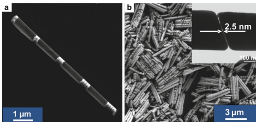
Fig. 10 Structures made by OWL. (a) Disk arrays (Adapted from [46]). (b) Zoomed out image demonstrating uniformity of rods [45]. (b inset) 2.5-nm gap produced by means of OWL [47, 48]
