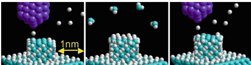
Fig. 17 (Left) H (white) atoms removed from Si (blue) surface by electron stimulated desorption by STM. (Middle) Si-H precursor gas selectively deposits on passivated Si where H has been removed (middle). (Right) Patterning process is repeated with another deposition cycle to create 3D structures
