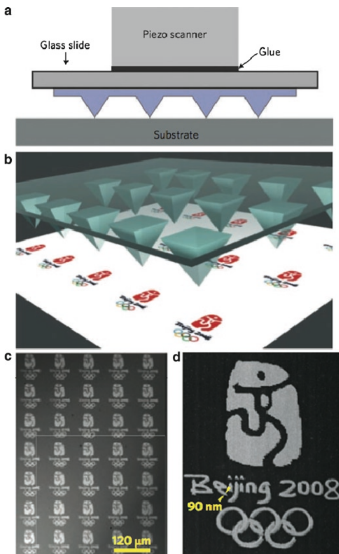
Fig. 7 (a) Scheme of the polymer pen array in a patterning instrument. (b) Scheme for fabricating the Beijing Olympic logo. (c) Optical micrograph of Au features showing high-throughput patterning. (d) Scanning electron micrograph where the smallest feature is 90 nm in diameter [41]
