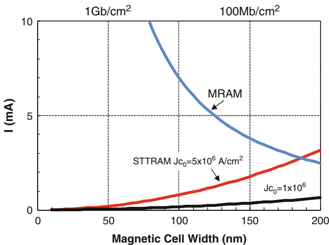
Fig. 3 Comparison of writing current scaling trends between MRAM and STTRAM (Wolf et al. [76])
