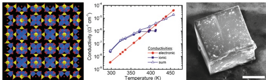
Fig. 21 (Left) Zeoate framework structure with [(As 6 VIV 12 VV 3 O 51 )–9Z] composition, where vanadium is blue, arsenic is yellow, and oxygen is red. The material crystallizes in a cubic space group with cell edge of 1,600 pm. (Middle) Plot of measured conductivities as a function of temperature (Data from [80]). (Right) Scanning electron micrograph of zeoate material from left panel; scale bar is 50 \mu\text{m} (Courtesy of V. Soghomonian, Virginia Polytechnic Institute and State University)
