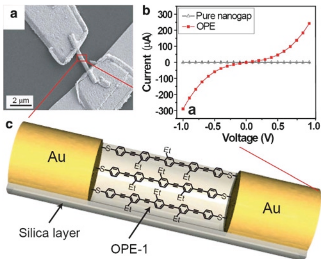
Fig. 11 (a) SEM image of a device prepared with an OWL-fabricated wire having a 3-nm gap. (b) Representative I - V response for 3-nm OWL-fabricated gaps before being modified with OPE-1 (Pure nanogap line) and after (OPE line). (c) A diagram of OPE-1 molecules spanning the 3-nm gap (Adapted from Chen et al. [50])
