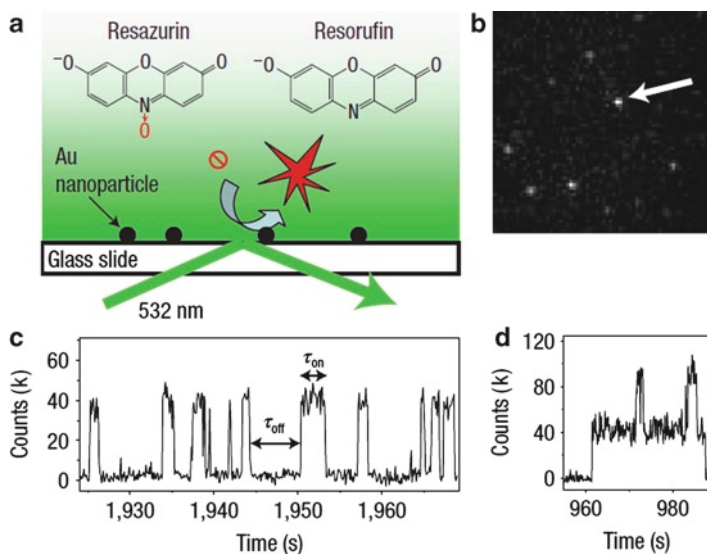
Fig. 5 Single-turnover detection of single-Au-nanoparticle catalysis. (a) Experimental design using total internal reflection fluorescence microscopy. (b) A typical image ( \sim 18 \times 18 \mu\text{m}^2 ) of fluorescent products during catalysis taken at 100 ms per frame. The pixel size is \sim 270 nm, which results in the pixelated fluorescence spots. (c) A segment of the fluorescence trajectory from the fluorescence spot marked by the arrow in b at 0.05 \mu\text{M} resazurin and 1 \text{ mM NH}_2\text{OH} . (d) A segment of another fluorescence trajectory showing two on-levels at the same conditions (From Xu et al. [26])
