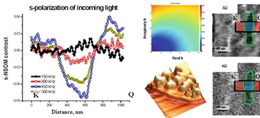
Fig. 12 The scattered NSOM signal profiles ( left ) and images ( right ) are compared to a model of the complex dielectric function of a molecular layer ( top, right ) and the topographic structure ( bottom, right ) [59]
