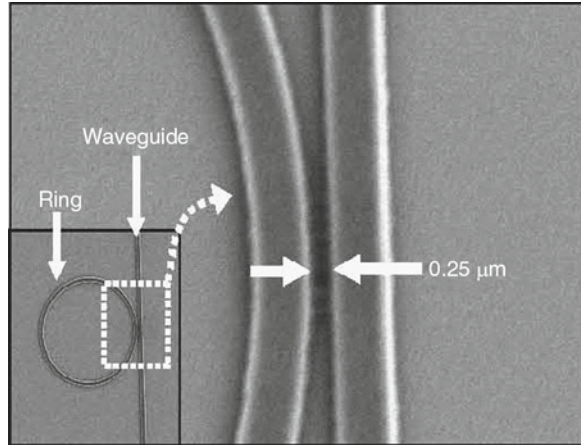
Fig. 5 SEM image of a Si-based ring resonator coupled to a waveguide. Inset shows the entire ring structure [44]
