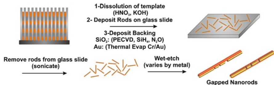
Fig. 9 The on-wire lithography (OWL) process [45]
