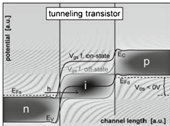
Fig. 6 Conduction and valence band for a p-type T-CNTFET in the on- and off-state. Holes are injected from the source for sufficiently negative gate voltages [85]
