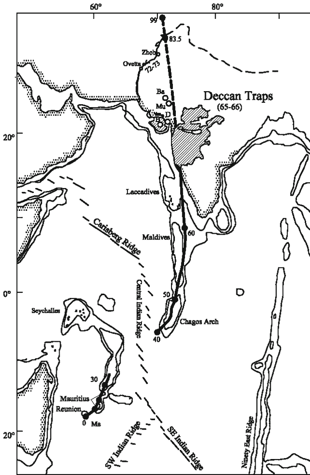
Fig. 10.16 The heavy line indicates the model 0–99 Ma track of the Reunion hotspot (Mahoney et al. 2002) assuming a stationary hotspot and that plate reconstruction are accurate. The dashed pre-Deccan portion is anchored by the 83.5 and 99 Ma plate reconstructions of Kent et al. (2002). The south Tethyan suture zone of Pakistan passes north and east into the Indus–Yarlung suture zone indicated schematically by the light dashed line . D: Dhandhuka, Ba: Botad, Ba: Barmer, Mu: Mundwara
