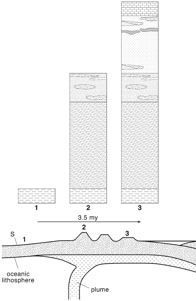
Fig. 1.8 Development of the stratigraphy of the Karmutsen Formation during the passage of a plate over an active plume. Clastic rocks containing Daeonella (1) were deposited before the plate passed over the stagnation point (S). The pillow basalt and subaerial basalts (2) were deposited by the time the plate passed over the plume centre, and the hyaloclastite and carbonate units (3) were deposited during subsidence and atoll development. Symbols are the same as in Fig. 1.2
