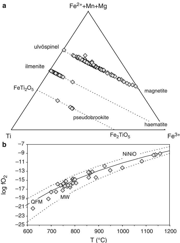
Fig. 7.7 (a) Diagram Fe–Ti–Mg–Mn (atoms) for the Deccan groundmass oxides (spinel, rhombohedral oxides and pseudobrookites); (b) T– fO_2 estimates for coexisting Fe–Ti oxides in the Deccan Traps. QFM = quartz–fayalite–magnetite buffer; WM = wustite–magnetite buffer, NiNiO = nickel–nickel oxide buffer
