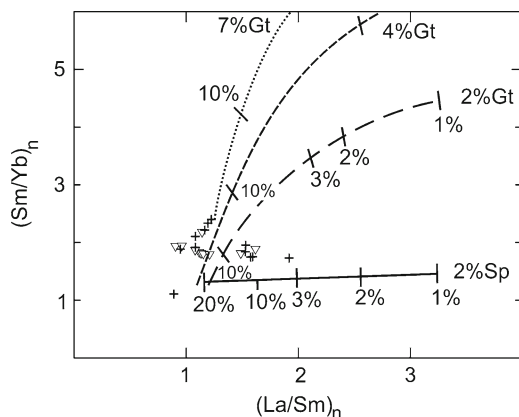
Fig. 1.7 Variation of chondrite-normalized Sm/Yb versus La/Sm ratios for the basaltic lavas ( crosses ) and non-cumulate subvolcanic mafic rocks ( triangles ) of the Karmutsen Formation. The non-modal batch melting curves for garnet and spinel peridotites are shown for comparison (Modified after Jourdan et al. 2007). The numbers and tick marks on the melting curves refer to percent partial melting. The modal composition of the garnet and spinel peridotite sources and mineral fractions in the liquids are after Jourdan et al. (2007). Source composition: 1.35 ppm La, 0.62 ppm Sm and 0.45 ppm Yb. Partition coefficients after McKenzie and O’Nions (1991). n – normalized to chondrites
