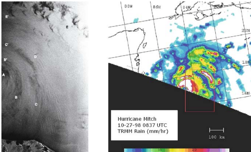
Fig. 4.6 RADARSAT-1 SAR ( left ) (copyright CSA) and TRMM ( right ) images from Hurricane Mitch on 27 October 1998. The SAR image at 1,133 UT covers 184 km \times 322 km. The TRMM image at 0837 UT has the same orientation as the SAR image and is 1,060 km \times 1,100 km. The red box outlines the SAR swath. The color scale is TRMM rainfall in mm/h. In the right panel : Green = 10 mm/h; red = 20 mm/h (from Katsaros et al., 2000)
