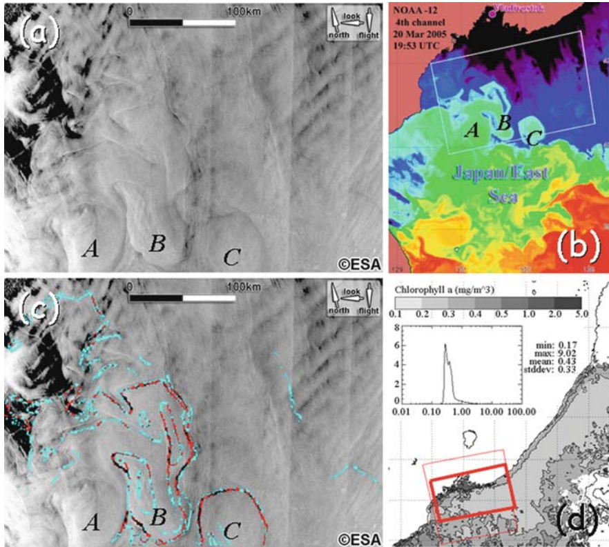
Fig. 7.2 Mesoscale eddies in the subarctic frontal zone of the Japan Sea on 20 March 2005: (a) ASAR image the size of 230 km \times 290 km taken at 12:50 UTC, (b) AVHRR infrared image at 19:53 UTC, (c) SST gradients superimposed on the same ASAR image and (d) map of chl- a concentration for 14–21 March. A white rectangle in (b) and the bold red rectangle in (d) mark the boundaries of the ASAR image
