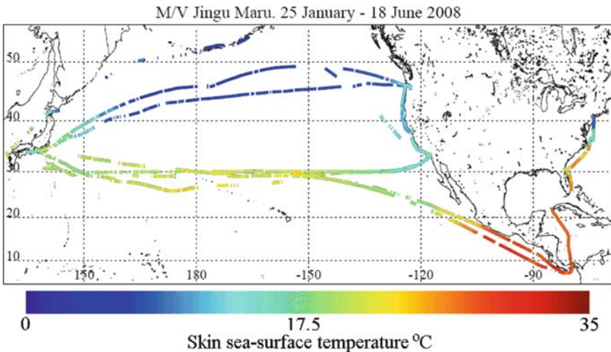
Fig. 14.3 Tracks of the M/V Jingu Maru between 25 January and 18 June 2008. The colors indicate the skin SST measured by an ISAR. Even though the cruise tracks are essentially zonal, they have sampled most of the SST temperature range in this period of about 6 months
