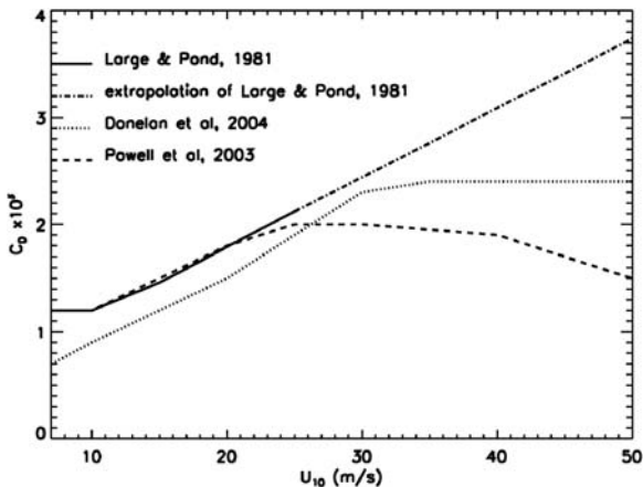
Fig. 6.3 Variation of the drag coefficients in strong winds
