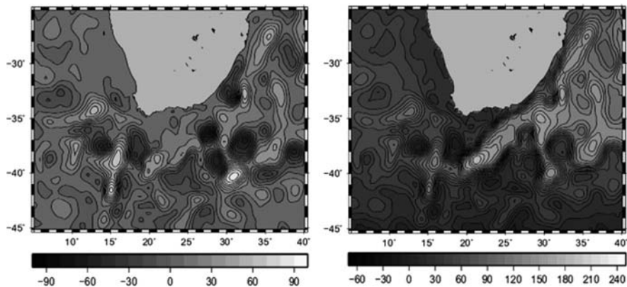
Fig. 10.7 Left : Sea level anomalies in the Aghulas current area on 18 February 2009. Right : matching absolute dynamic topography from CNES-CLS09 MDT
