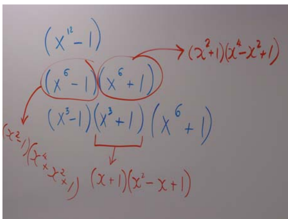
Fig. 5 Dan's counterexample in the central section, with the counterproposal by Paul that x^6 - 1 does indeed yield x^2 - 1 (at the leftmost arrow)
