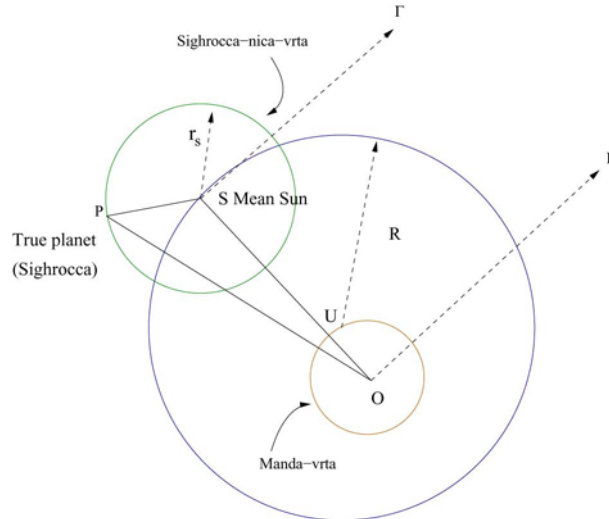
Fig. 2.4 Śīghra-samskāra for interior planets to obtain the geocentric longitude, prior to Tantrasaṅgraha
