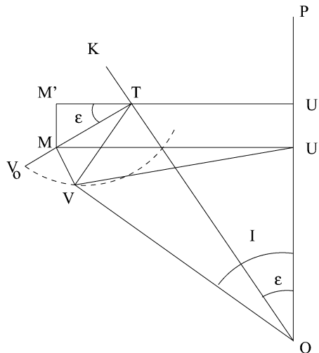
Fig. 2.11 The inclination of moon's orbit with the equator
