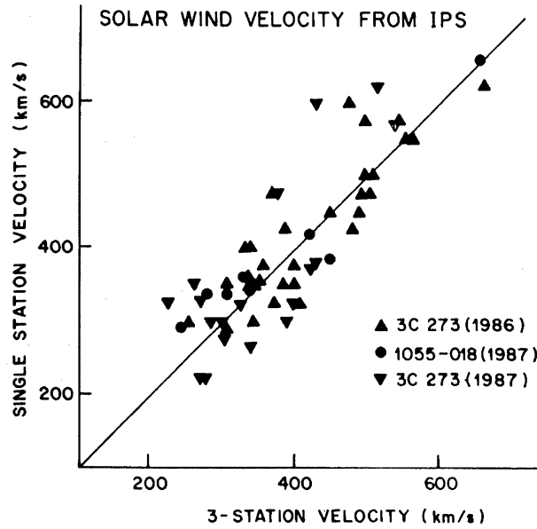
Fig. 5.14 Plot of solar wind velocity derived from single station IPS power spectra observations made with the ORT versus 3-station IPS system in Japan (Manoharan and Ananthkrishnan (1990))
