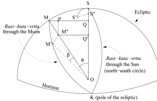
Fig. 2.12 Calculation of bimbantara , the distance between the solar and lunar discs
