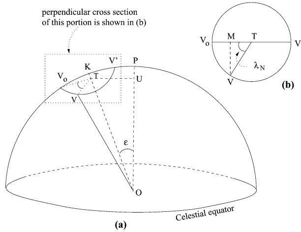
Fig. 2.10 The relative locations of the poles of the equator, ecliptic and moon's orbit
