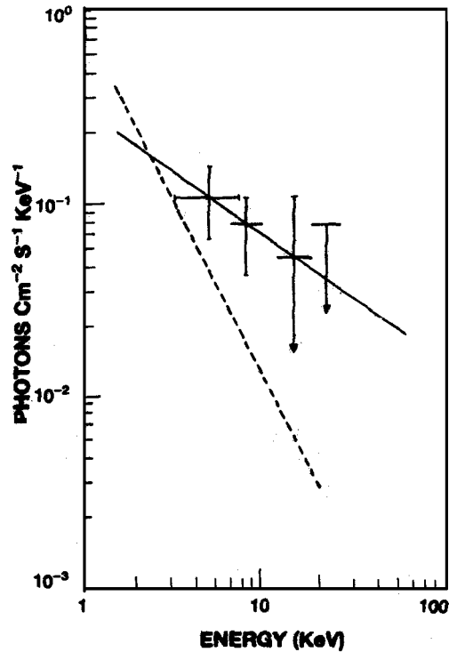
Fig. 4.5 Aryabhata observations on CygX-1 (thick line) before the intensity transition compared with the Aerial V observations (dotted line) after the transition. (K Kasturirangan, SC Chakravarty, MG Chandrasekhar. Science with Space Platforms- Indian Efforts in Retrospect & Prospects , in: Space - In Pursuit of New Horizons. A festschrift for Prof. UR Rao (eds. RK Varma, K Kasturirangan, US Srivastava, BH Subbaraya), Ind Acad Sci pp.155-181)
