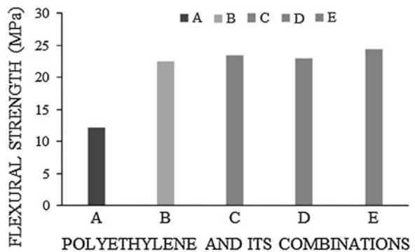
Fig. 3 Flexural strength of various PE specimens
