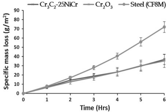
Fig. 6 Cumulative mass loss versus time plots for bare, D-gun \text{Cr}_3\text{C}_2\text{-}25\text{NiCr} and \text{Cr}_2\text{O}_3 coated CF8M steel at 2,250 rpm with slurry of 10,000 ppm concentration and average particle size 100 \mu\text{m}
