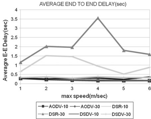
Fig. 9 E-E delay versus speed (TCP Traffic)
