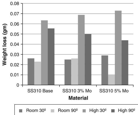
Fig. 4 Erosion results for hardfaced SS310 steel
