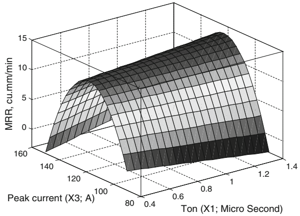
Fig. 7 Interaction effect of T_{ON} and peak current on MRR ( \text{mm}^3/\text{min} )
