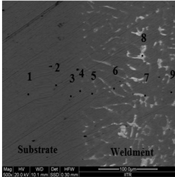
Fig. 1 Cross-sectional EDS point of SS310 steel hardfaced with alloy 3
