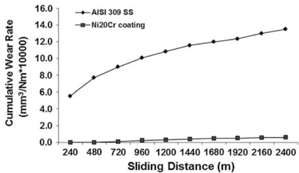
Fig. 3 Variation in CWR with sliding distance for the uncoated and plasma-sprayed Ni-20Cr-coated AISI 309 SS steel subjected to wear at normal load of 30 N and sliding velocity of 1 m/s
