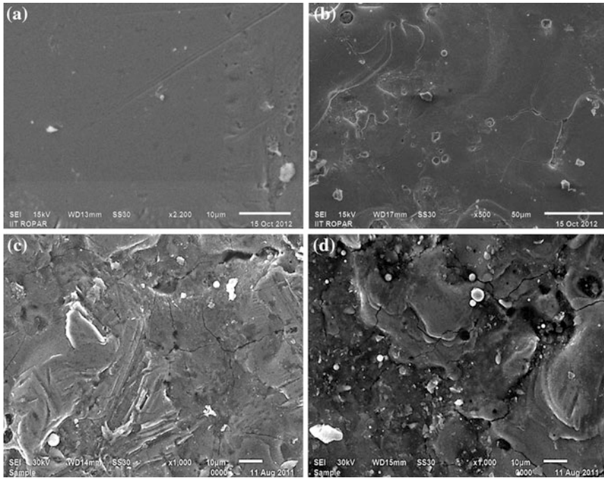
Fig. 7 Surface topography of samples machined by EDSG process, (a) 2,200×, (b) 500×, (c) grinding marks due to pronounced grinding effect (60 mesh SiC) at 1,500 rpm, (d) EDMed surface machined with die sinking at 8 A, 1,000×
