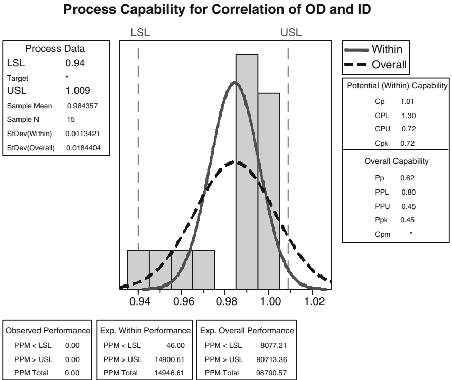
Fig. 5 Process capability for correlation of OD and ID
