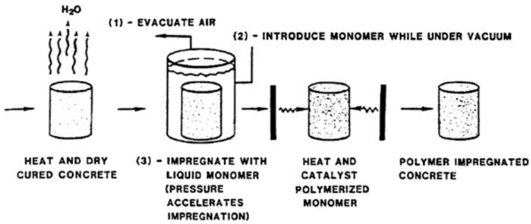
Fig. 1 Polymer concrete processing
