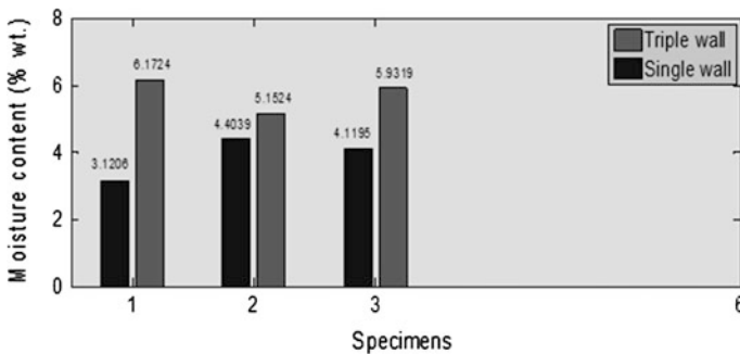
Fig. 2 Moisture content in plastic-coated corrugated board
