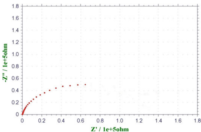
Fig. 10 Nyquist plot for the composite electrode sample aCN-WC
