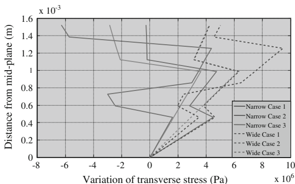
Fig. 3 Transverse stresses for the three lay-ups using both narrow- and wide-beam assumption
