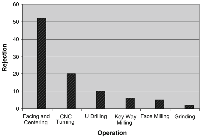
Fig. 2 Operation-wise rejection of the crankshaft P19
