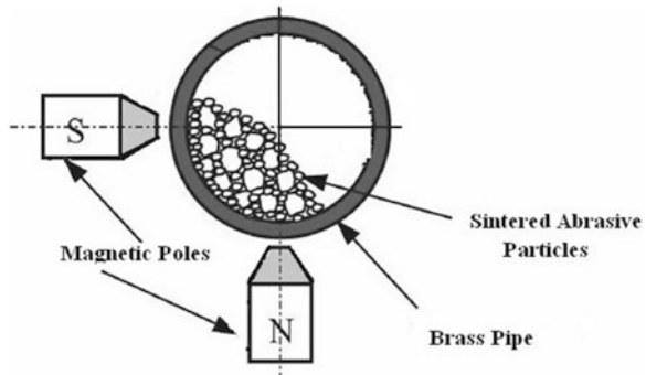
Fig. 1 Schematic of internal magnetic abrasive finishing
