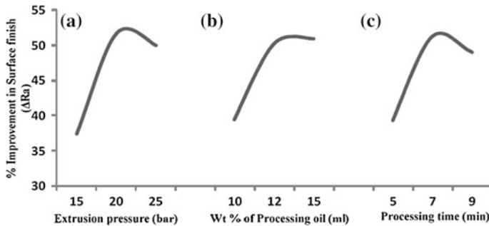
Fig. 4 Response curves showing the individual effect of process parameters on surface finish
