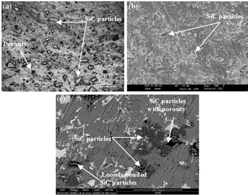
Fig. 4 a Optical micrographs, b SEM, c FE-SEM images of Al6063/10 % SiC composites reinforced with 15- \mu m-size SiC particles
