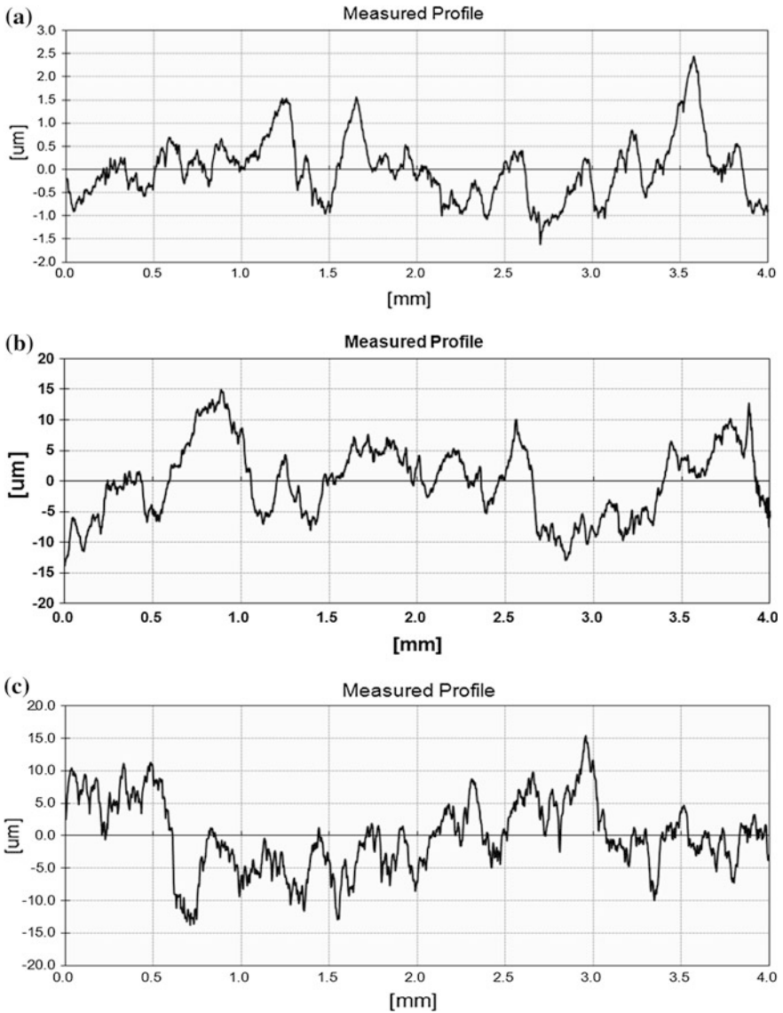
Fig. 5 Surface roughness profile of slurry eroded a \text{Cr}_3\text{C}_2\text{-25NiCr} coating, b \text{Cr}_2\text{O}_3 coating, and c CF8M steel
