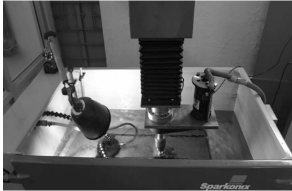
Fig. 2 Experimental setup of ED SG
