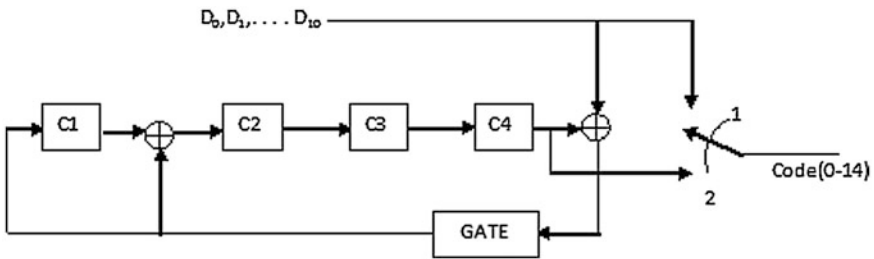
Fig. 16.1 Encoder for (15, 11) cyclic code
