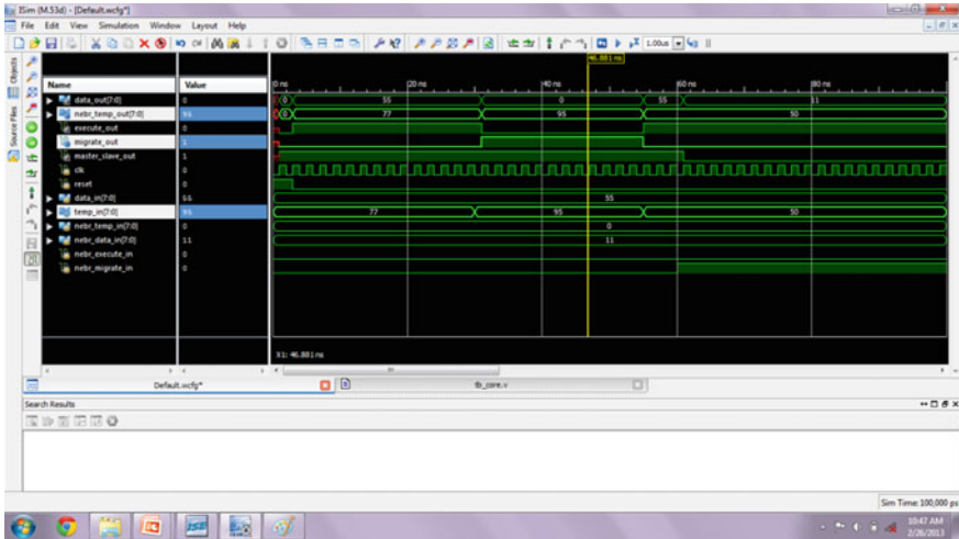
Fig. 14.5 Output waveform representing task migration in single core
