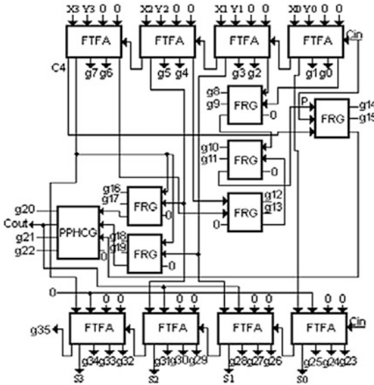
Reversible logic implementation of fault tolerant carry skip BCD adder.
