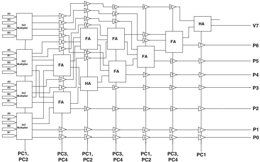
Fig. 15.4 Proposed 4 \times 4 adiabatic Vedic multiplier
