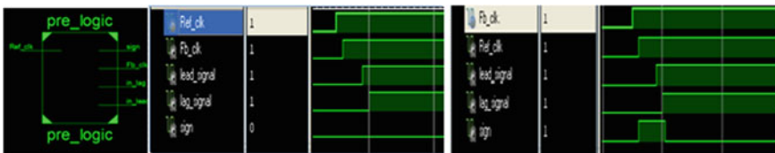
Fig. 18.4 Prelogic unit indicating positive and negative phase differences
