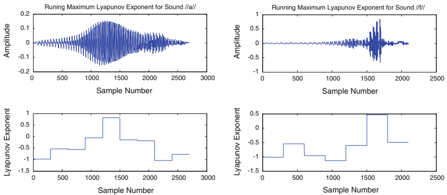
Fig. 42.3 Running maximum Lyapunov exponent for vowel sound “a” and running maximum Lyapunov exponent for sound “f”
