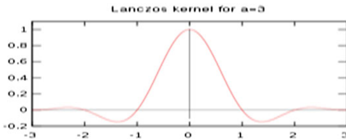
Fig. 48.1 Lanczos kernel for a = 3 [2]
