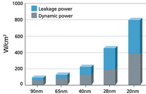
Fig. 20.1 Leakage power is becoming a significant component of total power consumption in nano-scaled technologies [1]
