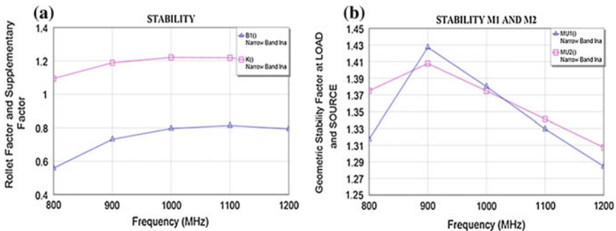
Fig. 26.3 a Shows Rollett’s stability factor ( K ) and supplemental stability factor ( B1 ) results, b Shows geometric stability factor MU1 (Load) and MU2 (Source)
