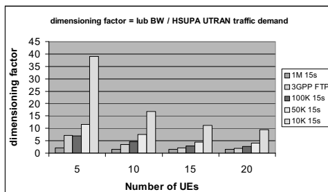
Figure A.18: Dimensioning factor
