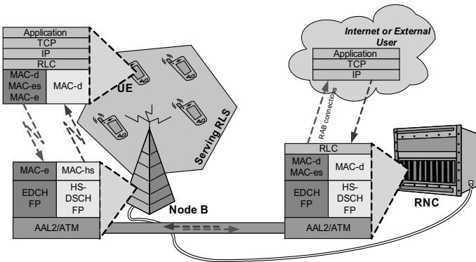
Figure A.9: HSPA simulator overview [LZK + 08]
