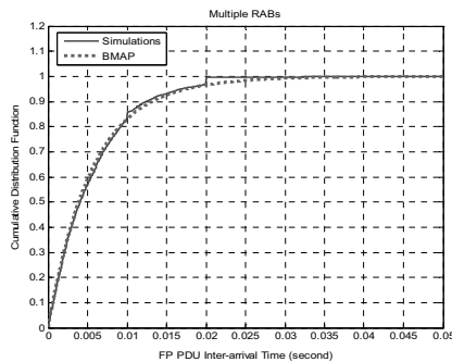
Figure 6.60: CDF of FP PDU Inter-arrival time – multiple RABs scenario
