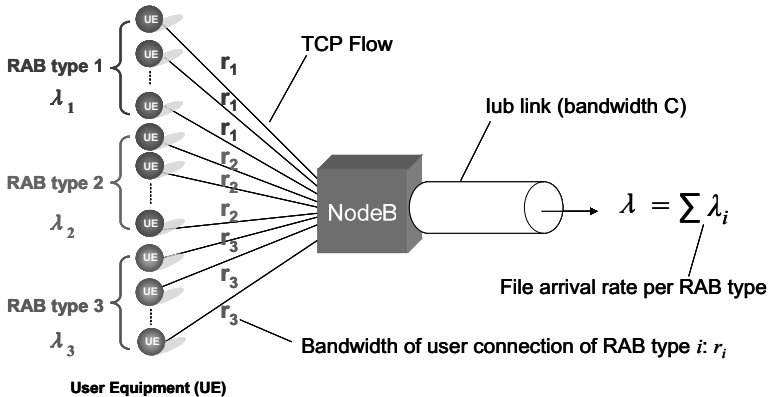
Figure 6.21: Flow level model for multiple RAB scenarios
