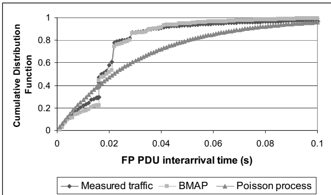
Figure 6.57: CDF of FP PDU inter-arrival time – single RAB scenario
