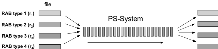
Figure 6.22: Processor Sharing
