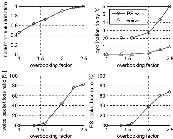
Figure A.32: Impact of overbooking
