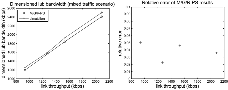
Figure A.29: Validating the dimensioning approach for the mixed traffic scenario for web traffic: RAB 128 kbps, no CAC, page size = 50 kbyte, delay factor f = 1.23 for voice traffic: AMR 12.2 kbps codec
