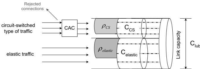
Figure 6.36: Bandwidth partitioning for elastic traffic & circuit-switched traffic
