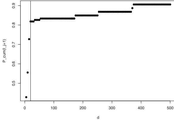
Fig. 3. Plot of cumulative probabilities P_{\text{cum}}(I_j = 1) across a range of distances d .
