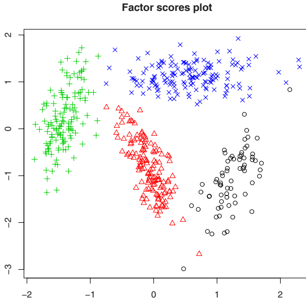
Fig. 1. Factor distribution.
