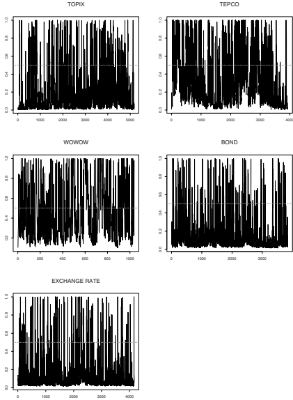
Fig. 3. Jump probability.
