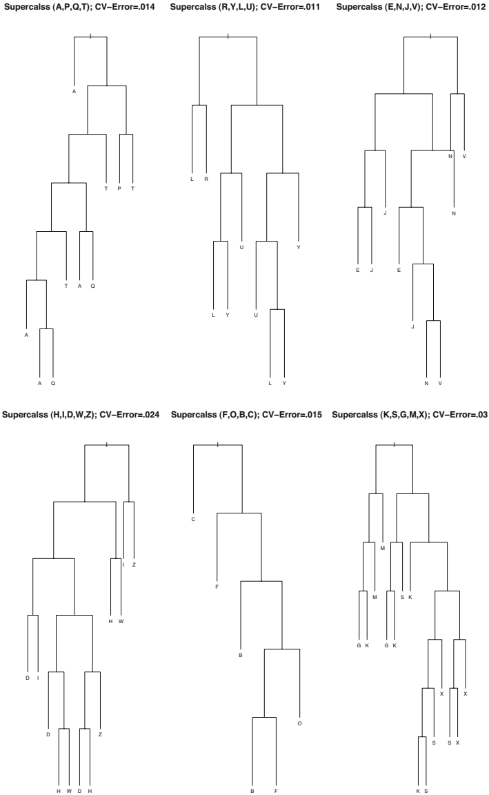
Fig. 2. The six classifiers obtained from the SASSC algorithm with g = 6 superclasses using the Gini splitting rule and 10-fold cross validation.
