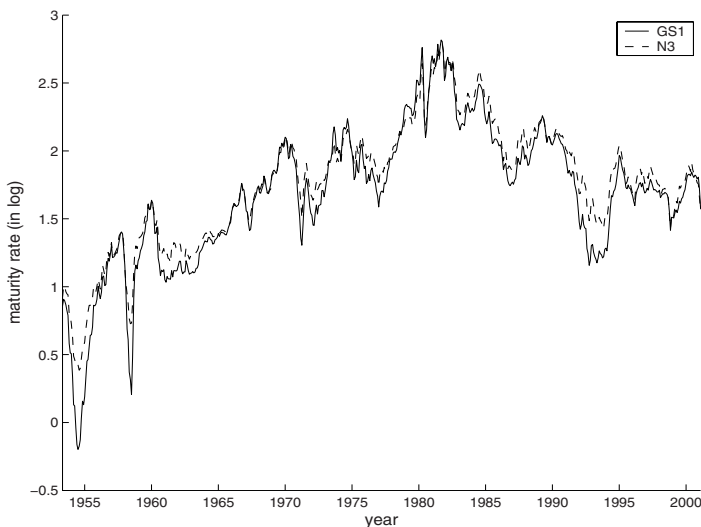
Fig. 1. Time plot of the “maturity rate” series. The solid line represents the 1-Year Treasury constant maturity rate and the dashed line the 3-Year Treasury constant maturity rate, both in logs.
