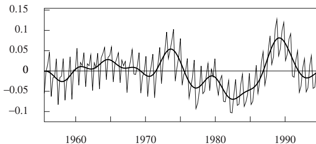
Fig. 9. The residual sequence from fitting a quadratic trend to the logarithmic consumption data. The interpolated line, which represents the business cycle, has been synthesised from the Fourier ordinates in the frequency interval [0, \pi/8] .
