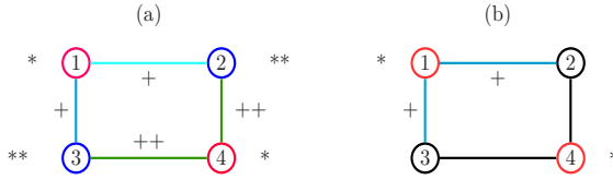
Fig. 1. Coloured graphs. (a): The edges 1:2 and 1:3 are in the same (light blue) edge colour class as also indicated by the “+”-sign. Likewise, 2:4 and 3:4 are in the same (green) edge colour class, also indicated by “++”. The vertices 1 and 4 are in the red vertex colour class (also indicated by “*”) while vertices 2 and 3 are in the blue vertex colour class (indicated by “**”). (b): Illustration of atomic colour classes. The vertices 2 and 3 are drawn in black and are atomic, so 2 and 3 are in different vertex colour classes. Likewise for edges 2:4 and 3:4.
