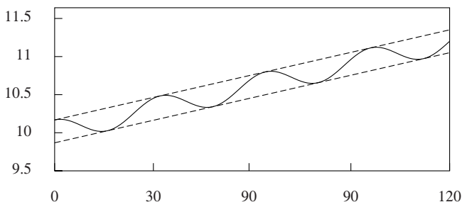
Fig. 2. The function \ln\{Y(t)\} = \ln\{\beta\} + rt + \gamma \cos(\omega t) representing the logarithmic business cycle data. The duration of the expansions and the contractions are not affected by the transformation.
