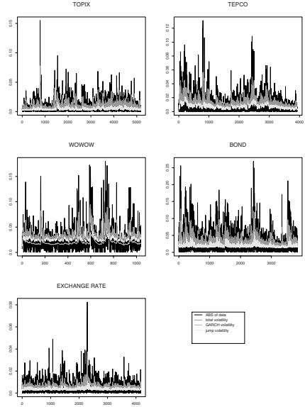
Fig. 5. Volatility.
