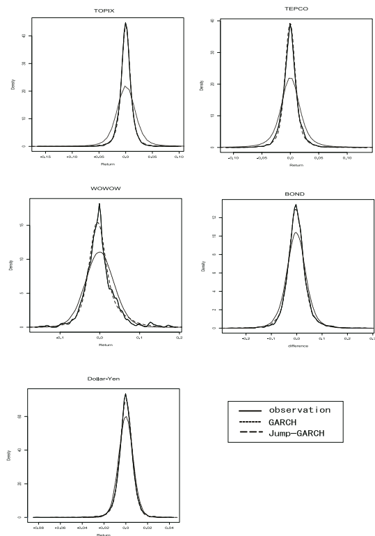
Fig. 1. Density.
