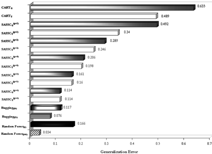
Fig. 1. The generalization errors for the Letter Recognition dataset provided by alternative approaches: as for SASSC, subscript G ( T ) indicates the Gini ( T woing) splitting rule, whereas apex g indicates the number of superclasses (i.e., classifiers) identified by the algorithm. The subscript for Bagging and Random Forest indicates the number of classifiers used to obtain the classification by majority voting.
