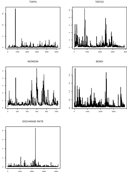
Fig. 2. Intensity.
