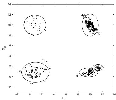
Fig. 5. BIC.
