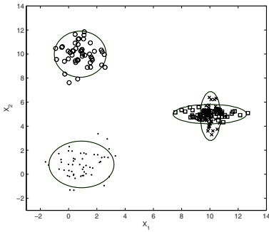
Fig. 2. BIC.
