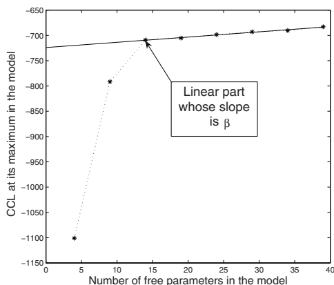
Fig. 1. Calibration of the slope.
