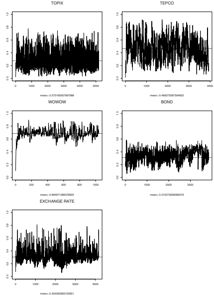
Fig. 4. Ratio of jump volatility.
