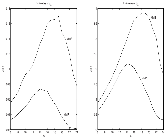
Fig. 2. MSE 's of MM-estimates for x_0 = 10 .
