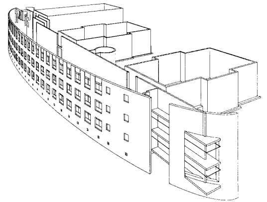
Conceptual perspective showing the new wall with existing teaching blocks behind
