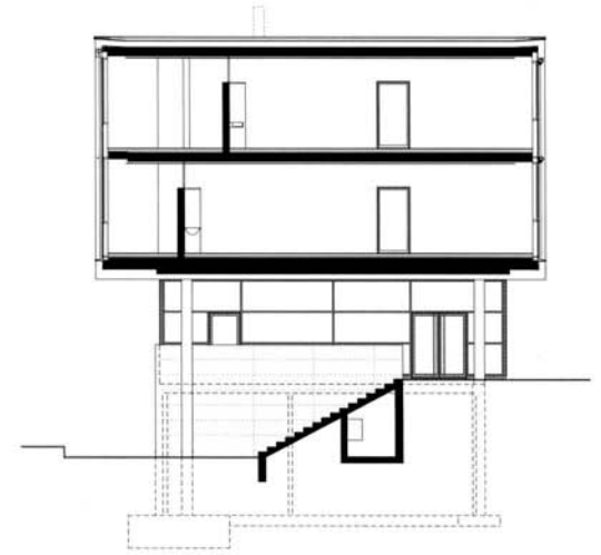
Cross section showing linking stair between lower and upper levels
