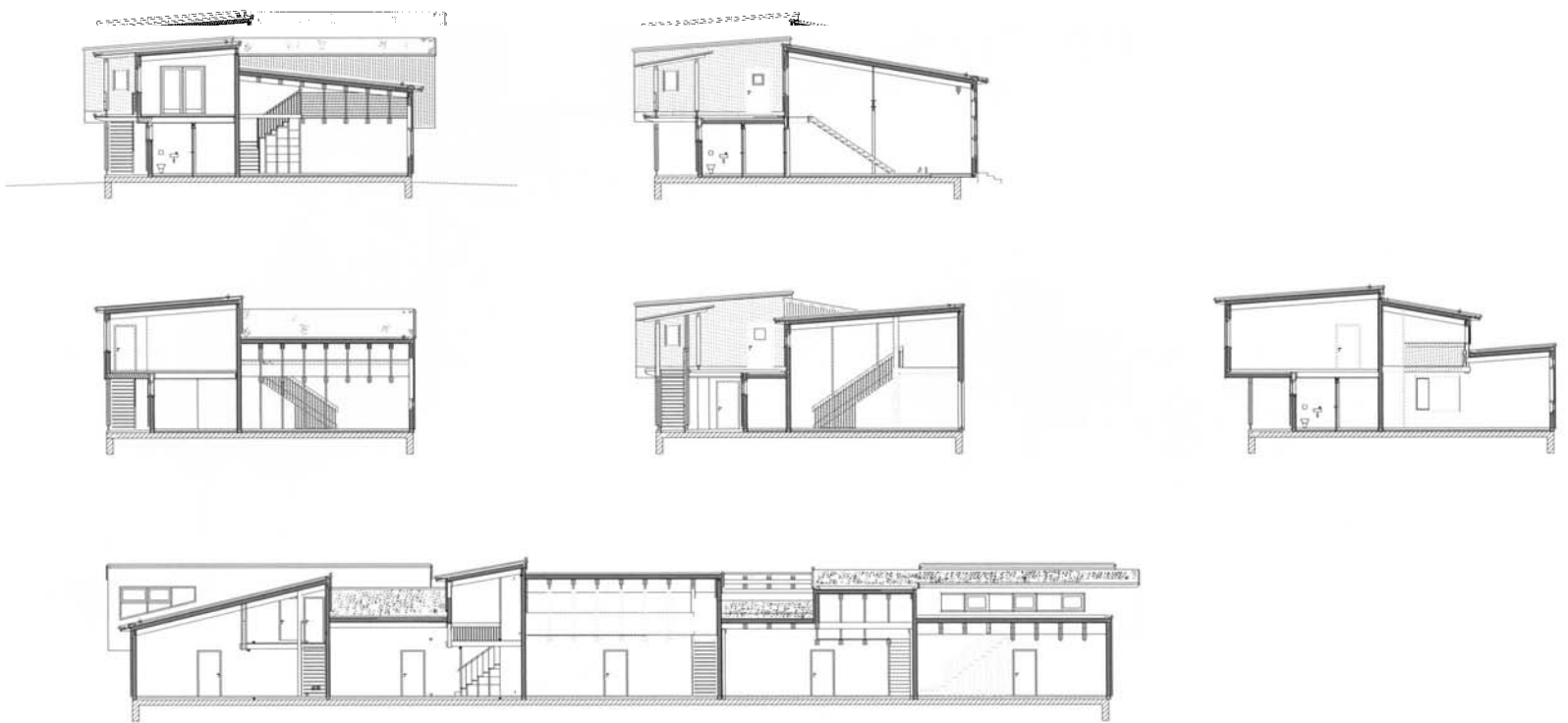
Sections
