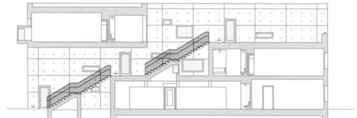
Section west-east
