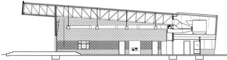
Section multi-purpose hall
