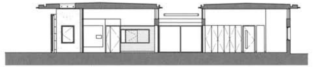
Sections looking north
