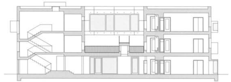
Section north-south
