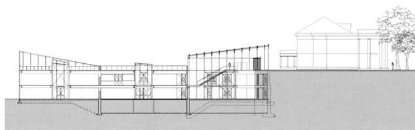
East-west section
