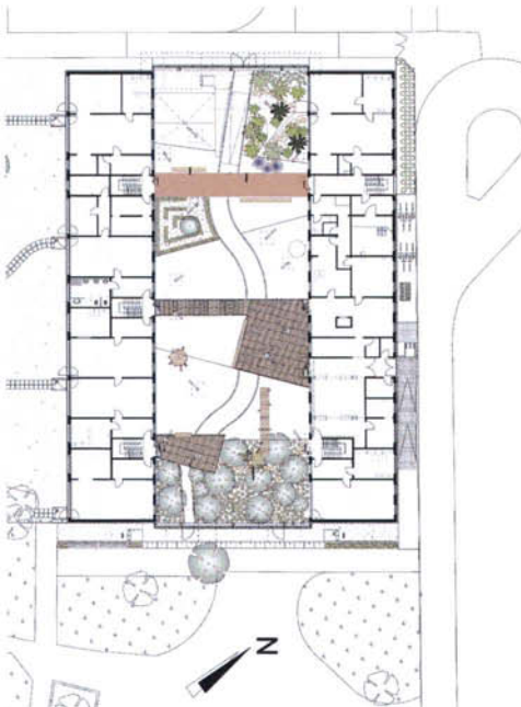
Daycare Centre 'Plappersnut' Wismar, Germany, refurbishment by IGEL-Planung, Martin Wollensak, Thomas Römhild, 2005
