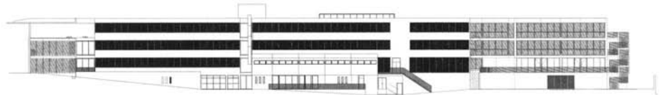
Main southeast elevation showing level changes
