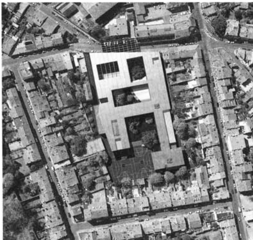
Aerial view | Games court with classrooms cantilevered above | First floor courtyard with the mature oak tree | An internal corridor with coloured light filtering through perimeter windows
