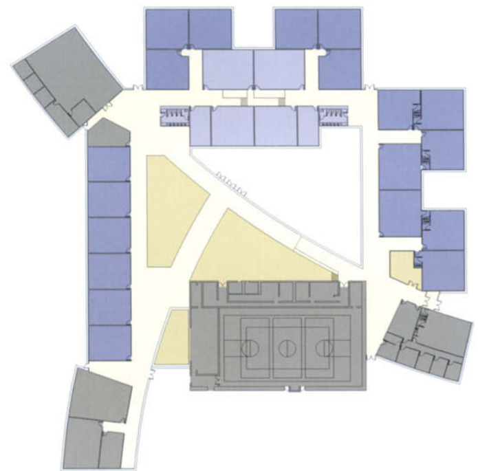
Plan showing public spaces at the key locations on the perimeter. Glenville Elementary School, Greenwich, Connecticut, Perkins Eastman Architects
