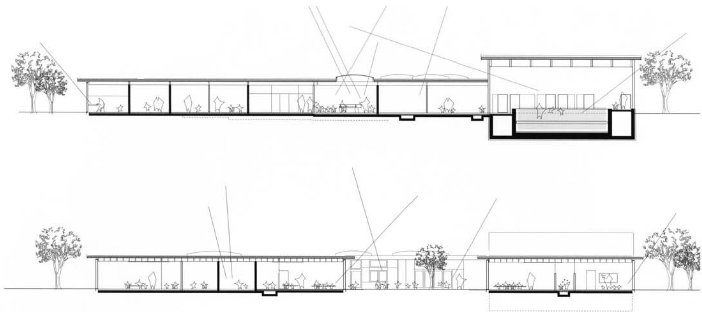
Section through classroom and community spaces
