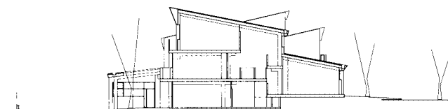
Section BB
