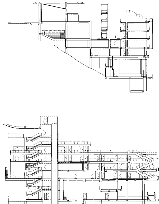
Sections
