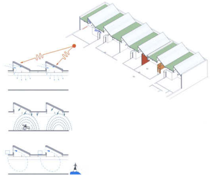
Daylighting concept
