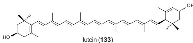
lutein (133)
