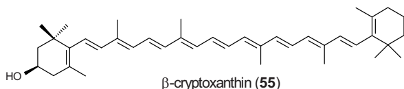
\beta -cryptoxanthin (55)
