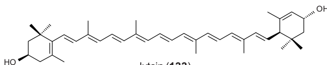
lutein (133)
