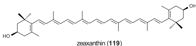
zeaxanthin (119)
