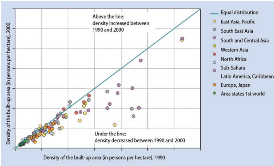
Fig. 3.12 Population density of 120 cities in a global sample in the period from 1990 to 2000 (Angel et al. 2011)
