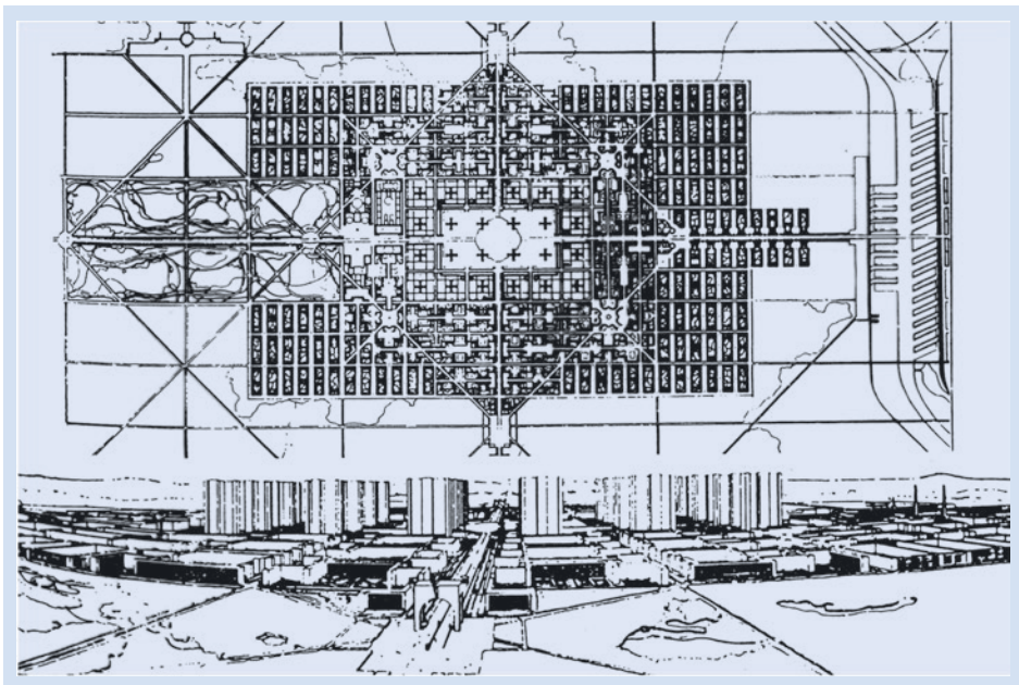
Fig. 7.4 A contemporary city for 3 million inhabitants, general view (Le Corbusier 1922)
