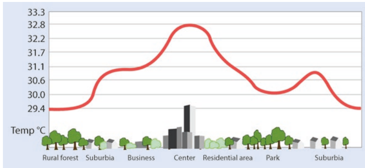
Fig. 5.6 Schematic representation of the urban heat island along a rural-urban gradient taking into account different land uses. (Kuttler 2000)
